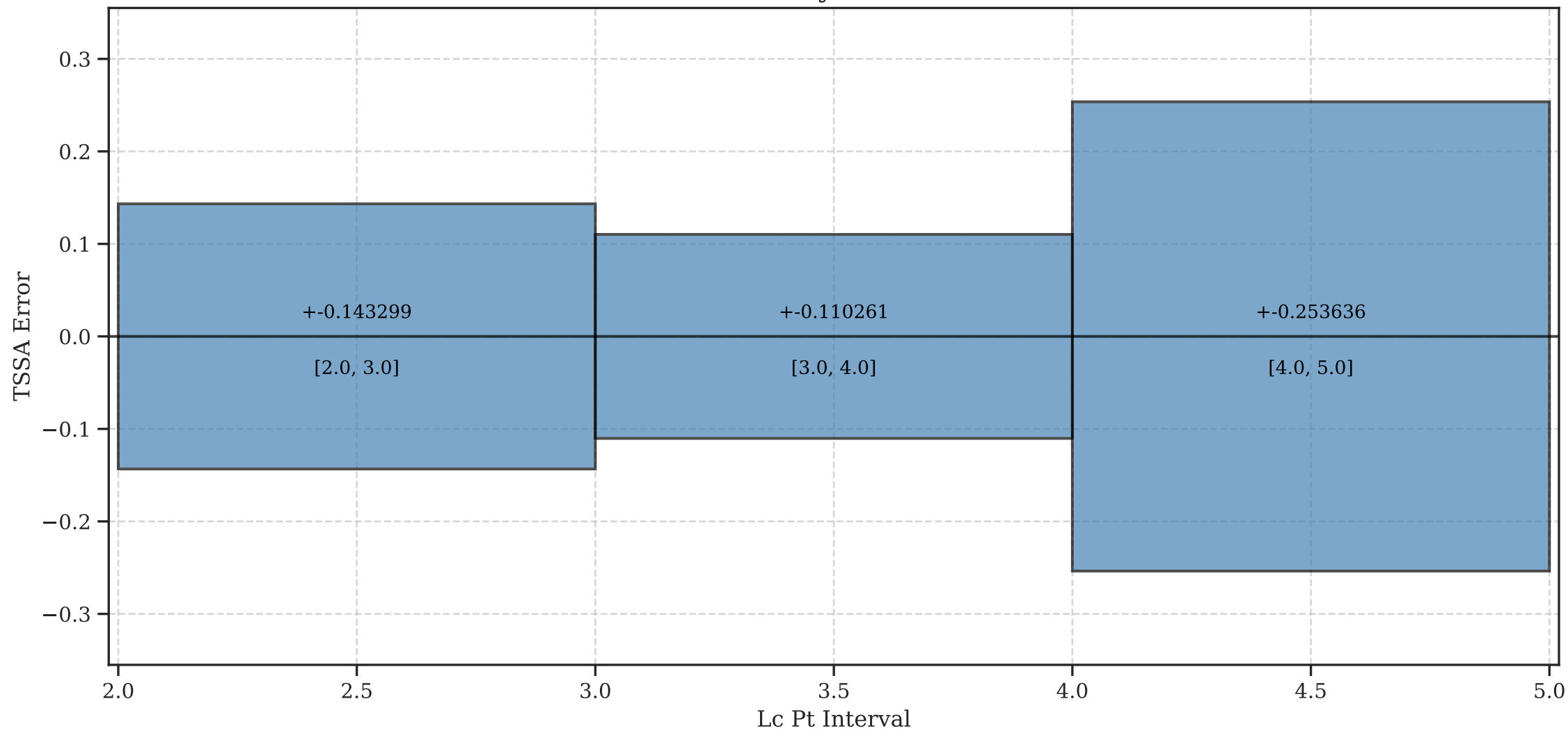
TSSA Error by Lc Pt Interval
