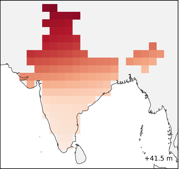
ERA5 (obs)
