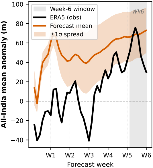
SPIRE
