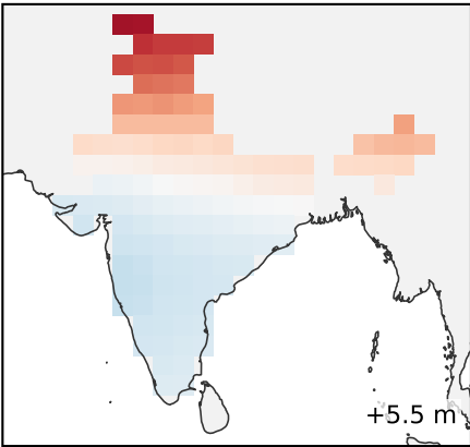
NCEP
