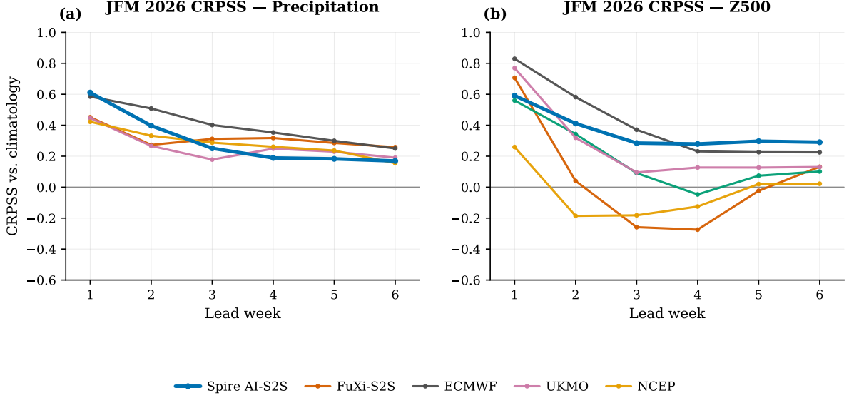
Figure 2: JFM 2026 all-India CRPSS versus lead week for precipitation (left) and Z500 (right). Positive values indicate probabilistic skill above climatology.
