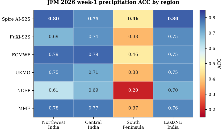
Figure 4: JFM 2026 week-1 precipitation ACC by IMD homogeneous region.
