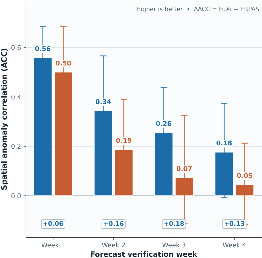
A ACC: anomaly-pattern skill
