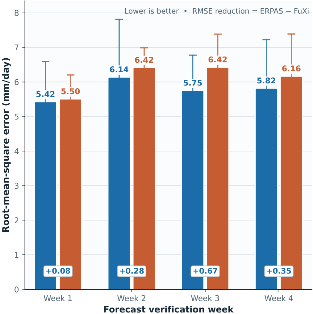
C RMSE: large-error sensitivity
