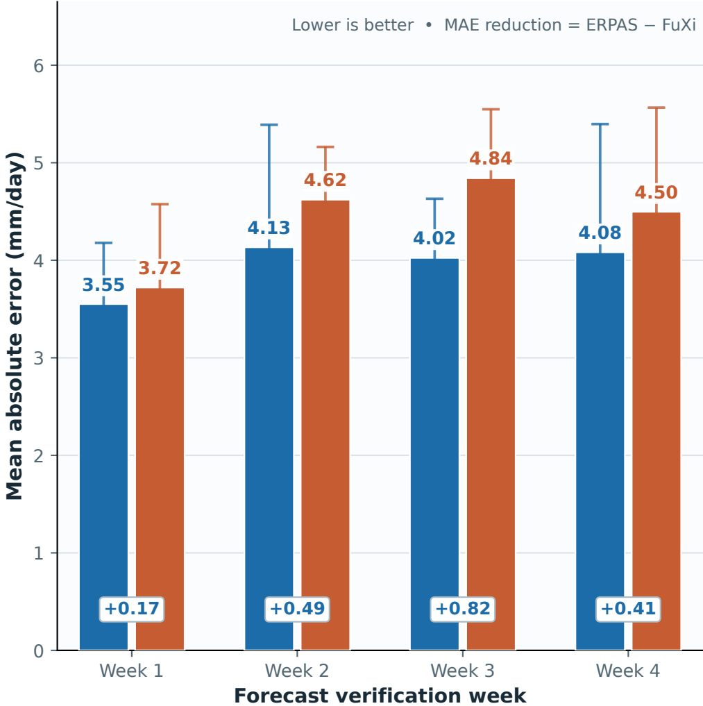
B MAE: rainfall-magnitude error
