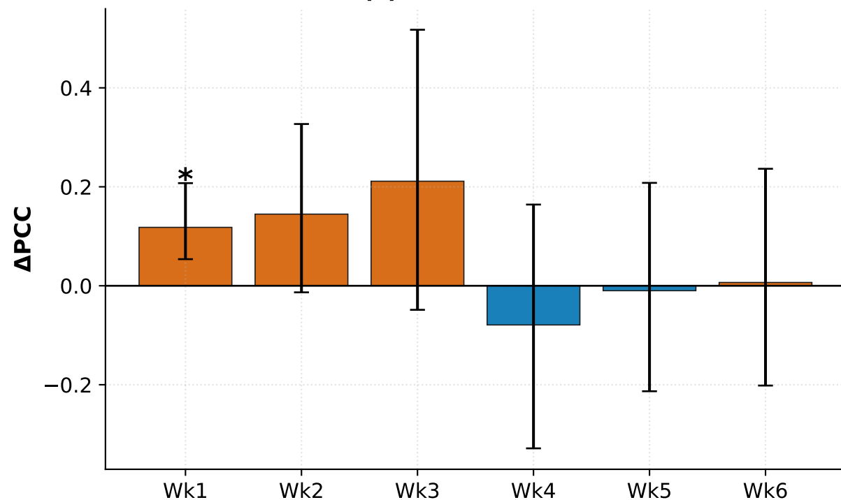
(c) Z500 — \Delta PCC
