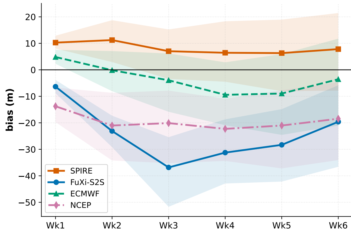
(a) Z500 mean bias
