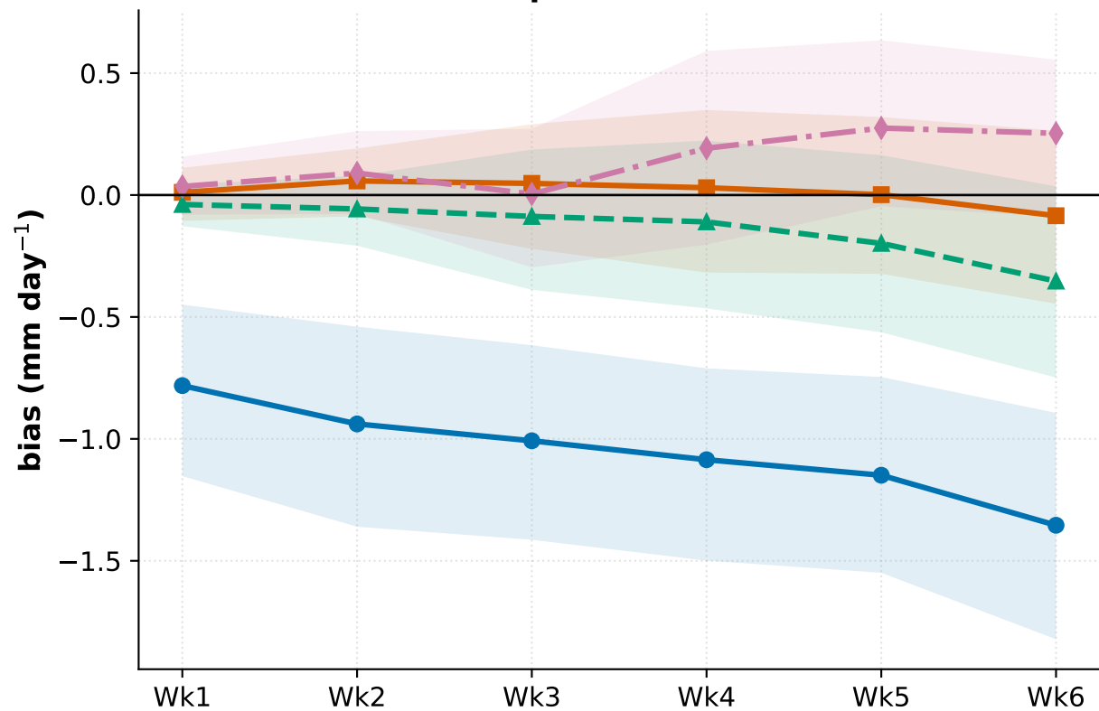
(b) Precipitation mean bias
