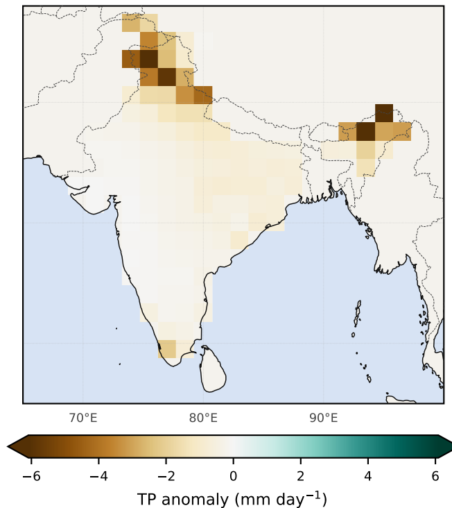
(b) Total precipitation anomaly
