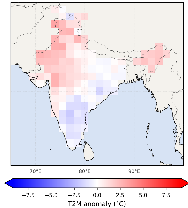
(c) 2 m temperature anomaly
