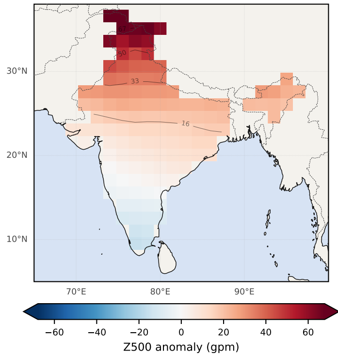
(a) Z500 height anomaly
