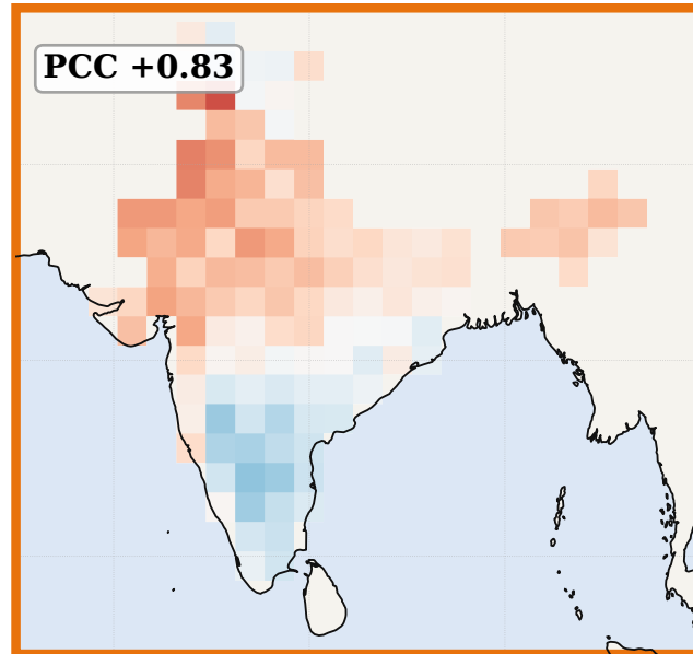
SPIRE
