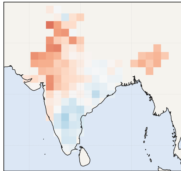
ERA5 (Obs)
