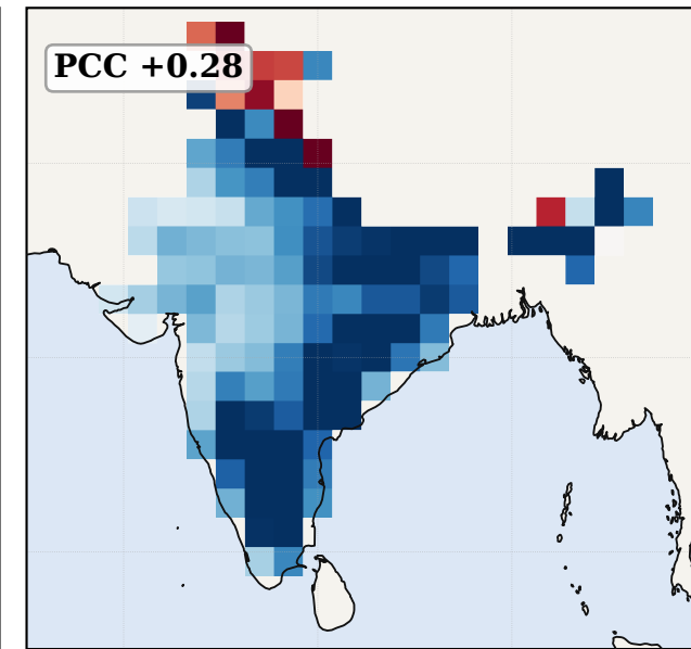
NCEP
