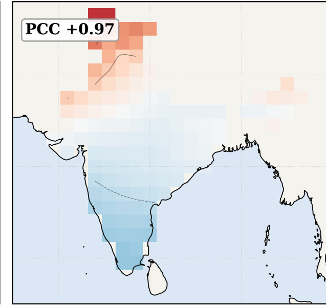
NCEP
