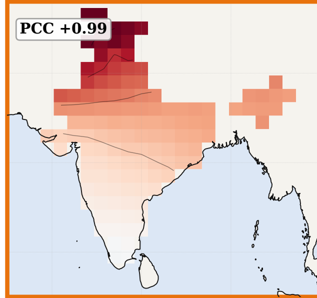
SPIRE
