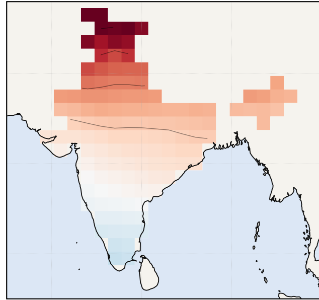
ERA5 (Obs)
