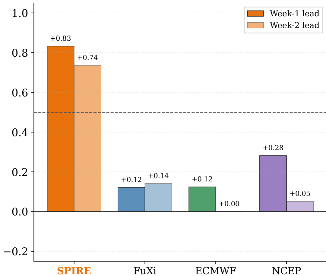
(a) T2M — PCC
