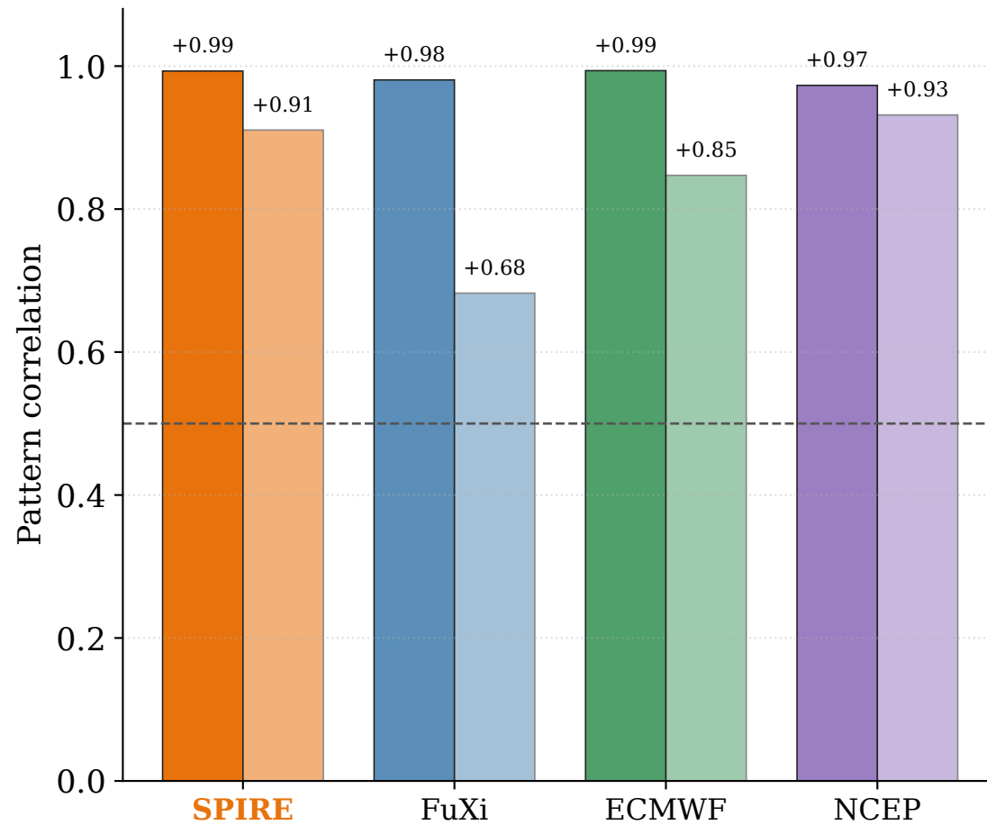
(b) Z500 — PCC
