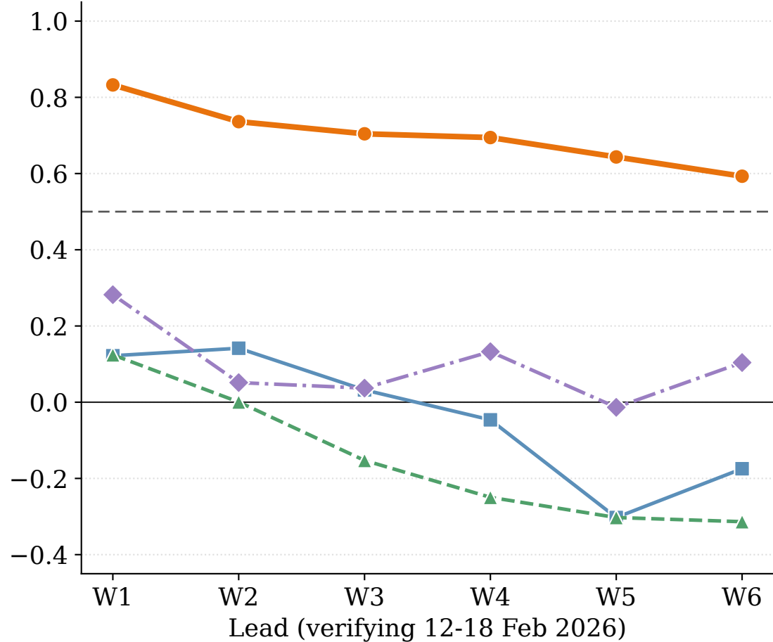
T2M anomaly PCC
