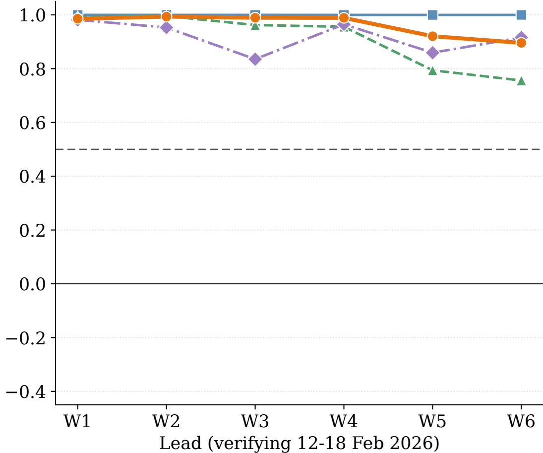
Precip anomaly PCC
