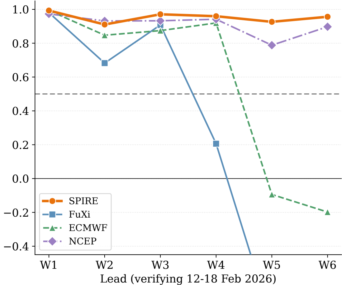
Z500 anomaly PCC
