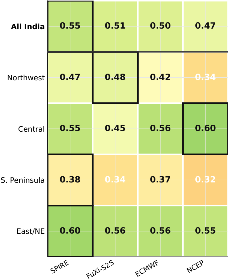
(a) Precipitation
