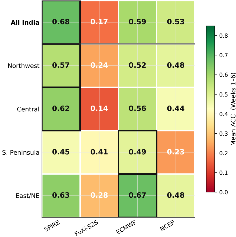
(b) Z500
