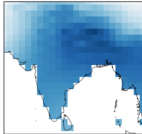
NCEP
