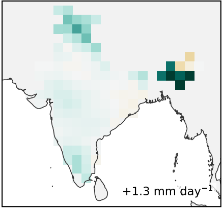
NCEP
