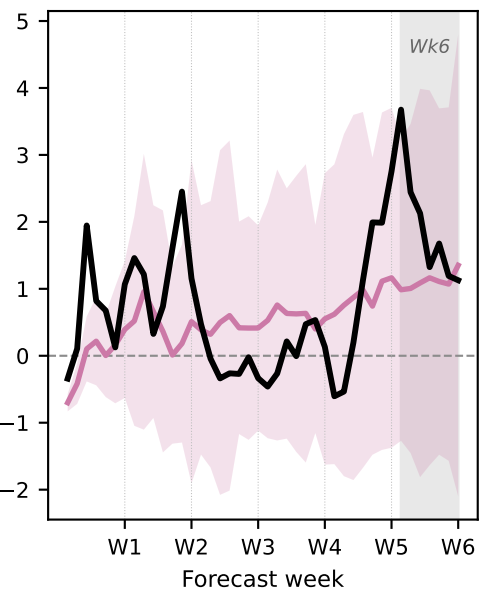
NCEP
