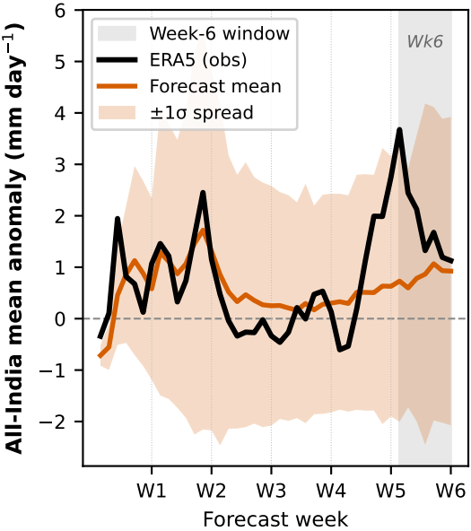
SPIRE
