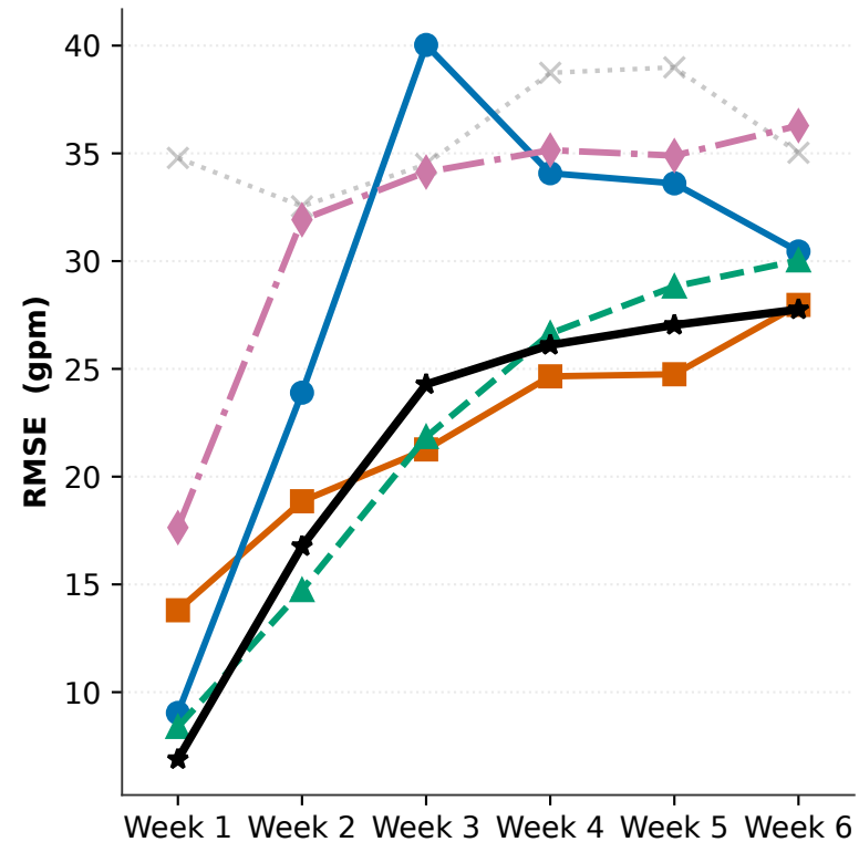
(c) Z500 — RMSE
