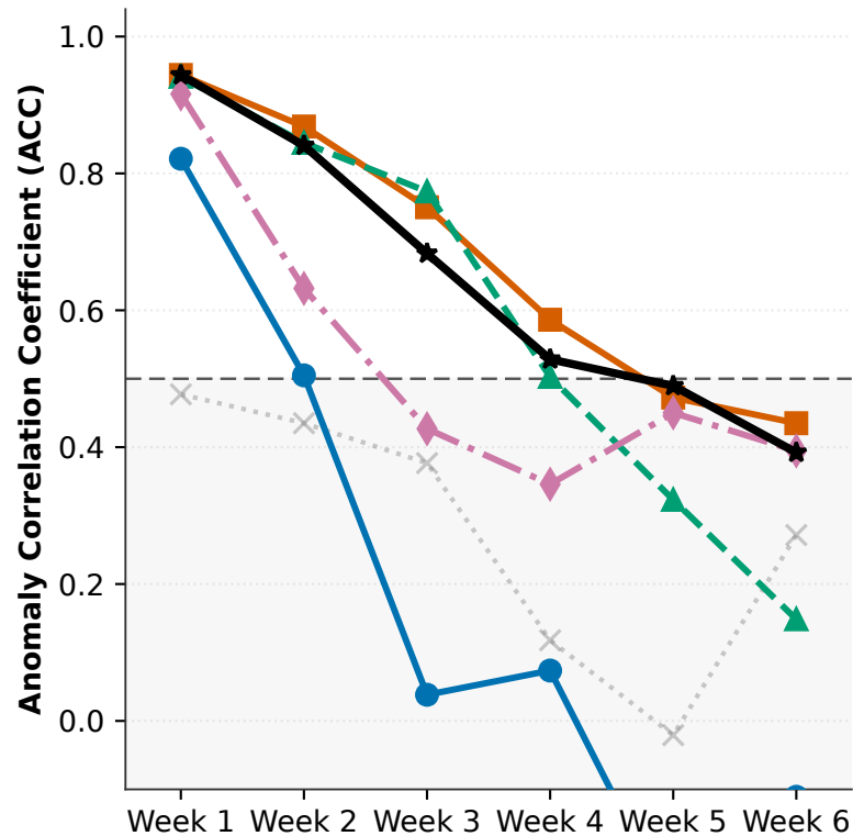
(b) Z500 — ACC
