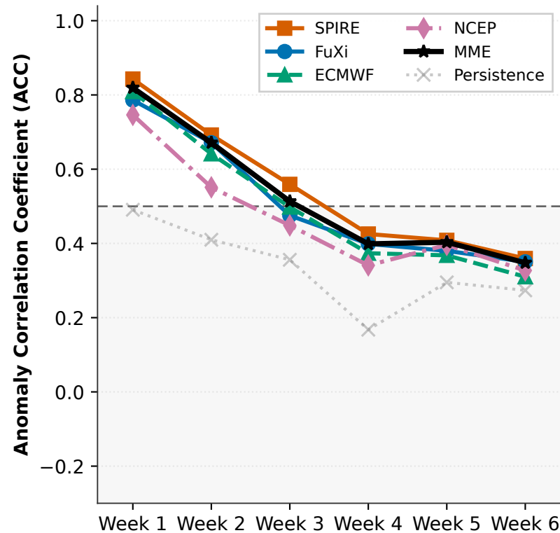
(a) Precipitation — ACC
