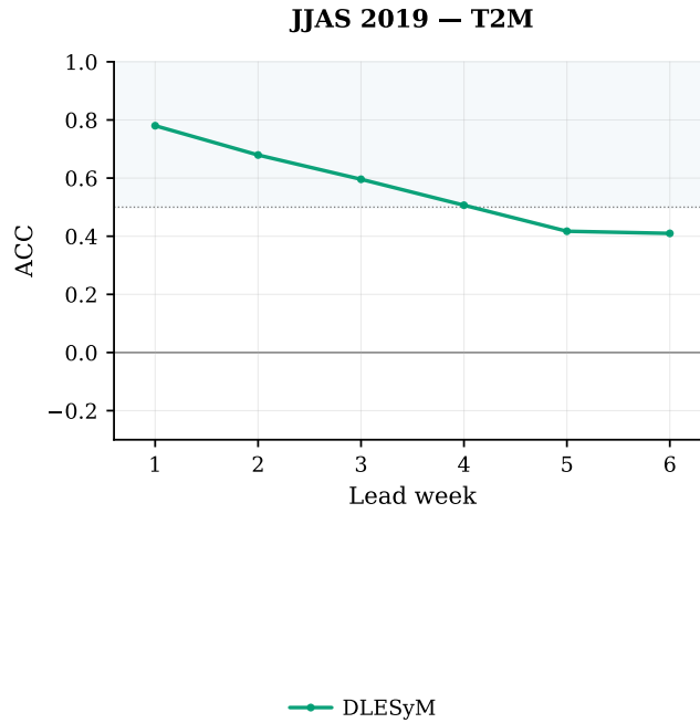
Figure 8: JJAS 2019 all-India T2M ACC versus lead week (DLESyM only; the only system with a scoreable T2M product in this season).
