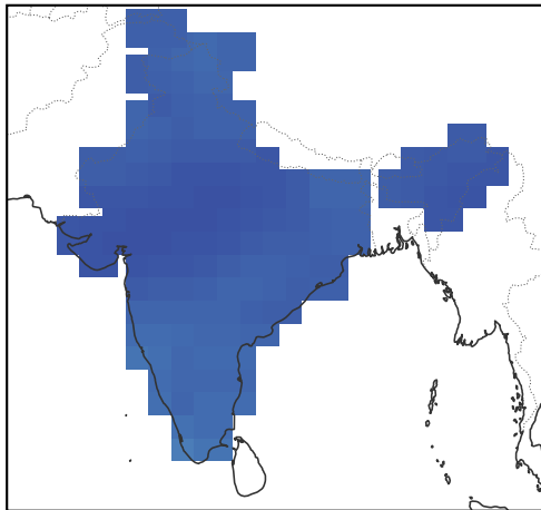
Spire AI-S2S
