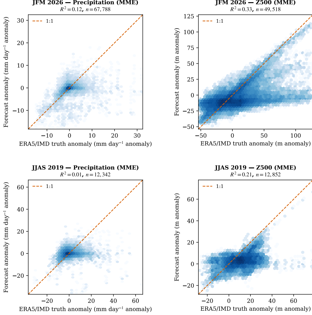
Figure 8: Forecast versus observed weekly anomaly for the multi-model ensemble (MME), pooled over all grid cells, lead weeks 1–6, and initializations. Hexbin shading shows point density (log scale); the dashed line is the 1:1 reference. R^2 is the squared Pearson correlation of the pooled pairs.
