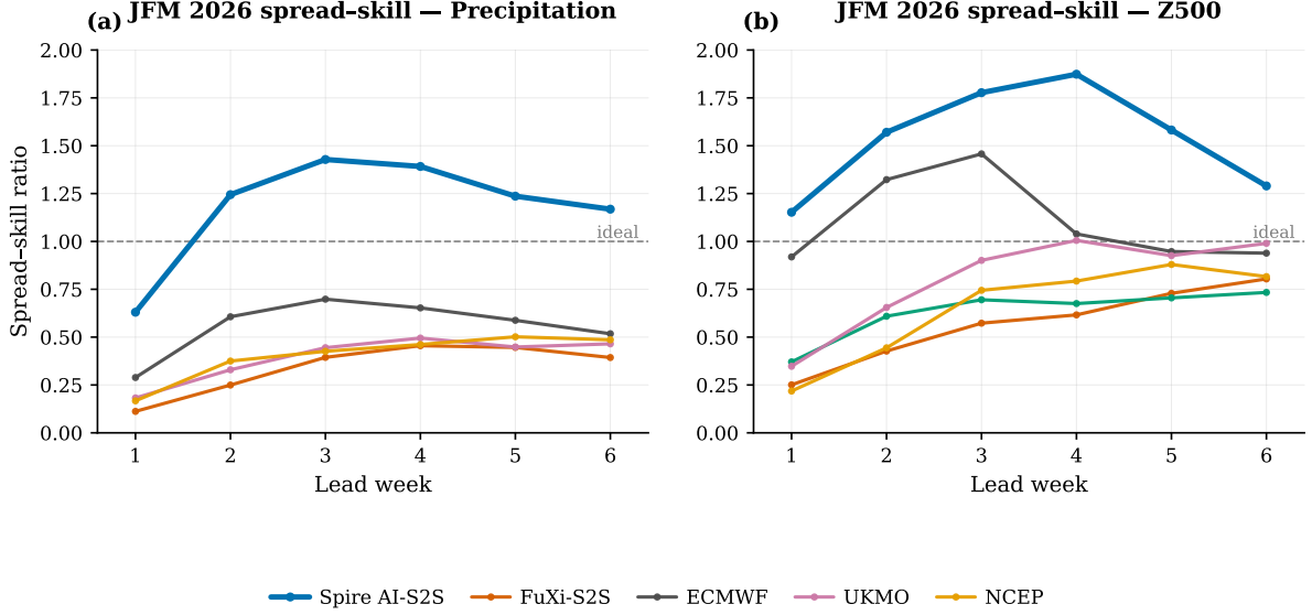
Figure 4: JFM 2026 spread-skill ratio versus lead week; a well-calibrated ensemble lies near unity (dashed line). Values < 1 indicate under-dispersion (overconfidence).
