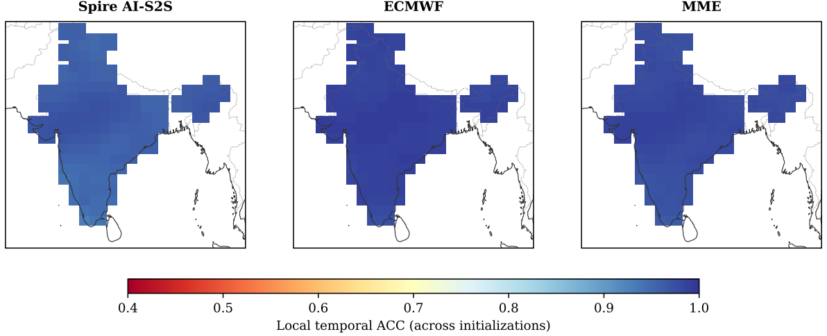
Figure 7: As Figure 6 but for week-1 Z500 anomaly. Note the different color scale (0.4–1.0 versus -0.4 –1.0 for precipitation), reflecting the much higher and more spatially uniform circulation skill.
