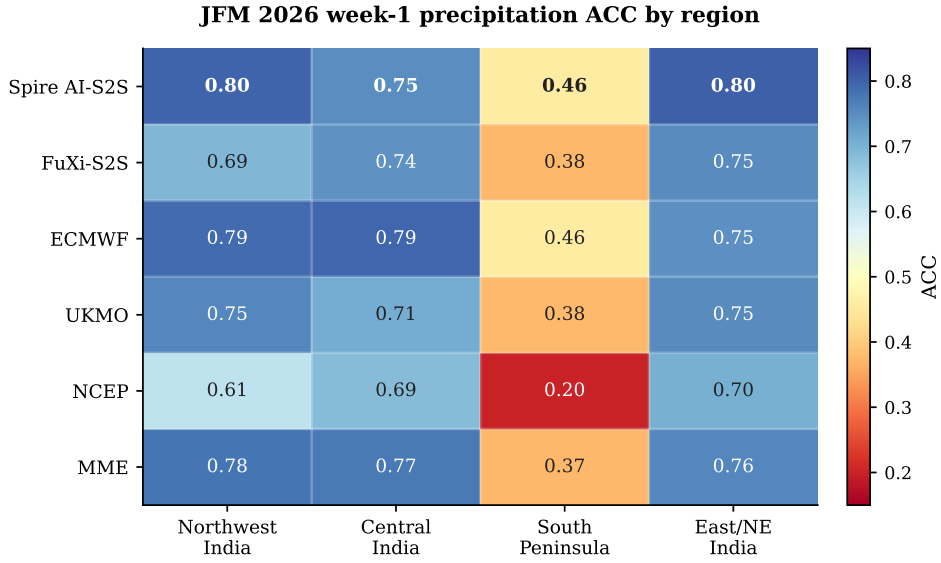
Figure 5: JFM 2026 week-1 precipitation ACC by IMD homogeneous region.
