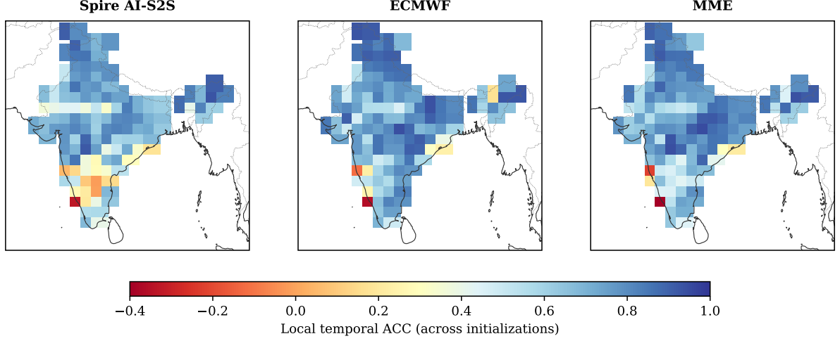
Figure 6: Local temporal ACC (Pearson correlation across the 90 JFM 2026 initializations) for week-1 precipitation anomaly at each 1.5^\circ grid cell, for Spire AI-S2S, ECMWF, and the multi-model ensemble (MME). All three systems are weakest over the southern tip of the peninsula.
