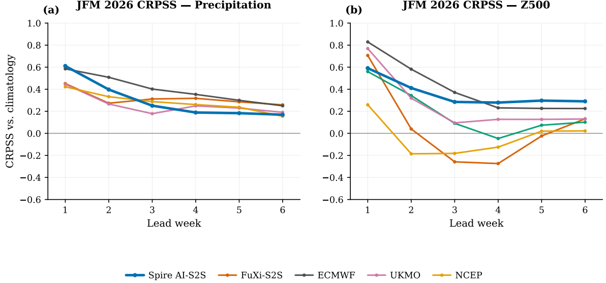
Figure 3: JFM 2026 all-India CRPSS versus lead week for precipitation (left) and Z500 (right). Positive values indicate probabilistic skill above climatology.
