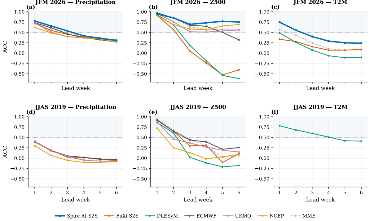
Figure 2: All-India anomaly correlation (ACC) versus lead week for six S2S systems. Top row: JFM 2026 (winter); bottom row: JJAS 2019 (monsoon). Columns: precipitation, Z500, 2-m temperature. Dotted line ACC= 0.5; solid line ACC= 0. DLESyM provides no precipitation; UKMO and ECMWF T2M are unscorable (single-step archive files, Section 7); NCEP has no T2M channel in this archive; Spire is unavailable for JJAS.
