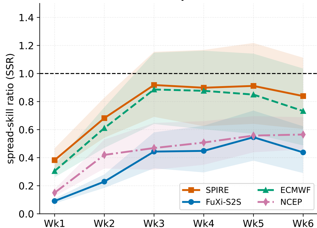
(a) Precipitation
