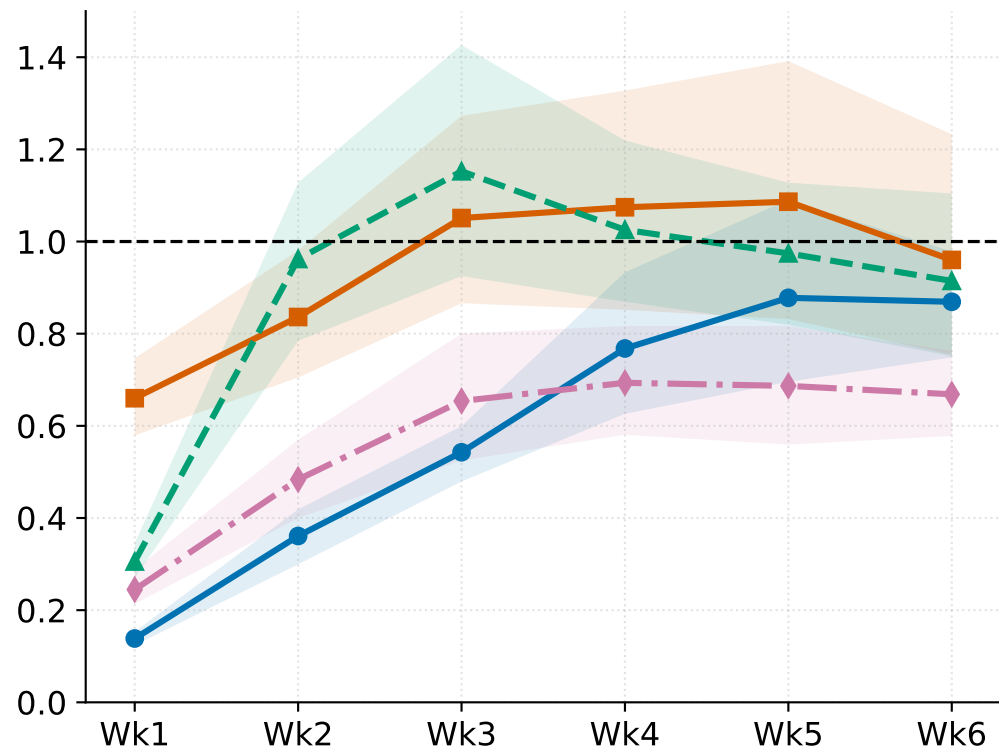
(b) Z500
