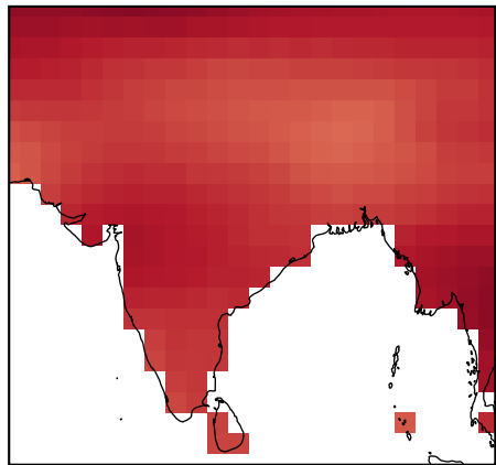
SPIRE
