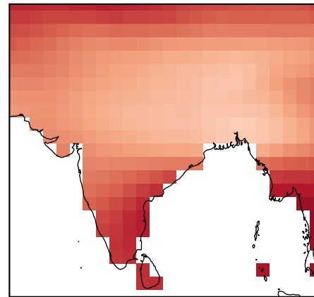
NCEP
