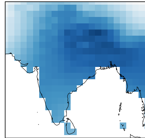
NCEP
