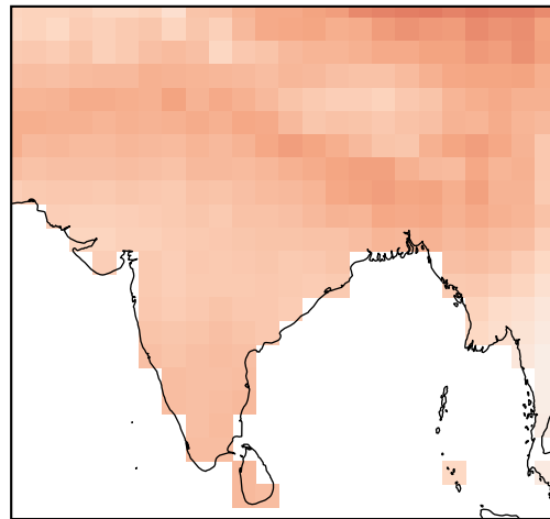
SPIRE
