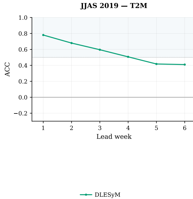
Figure 6: JJAS 2019 all-India T2M ACC versus lead week (DLESyM only; the only system with a scoreable T2M product in this season).
