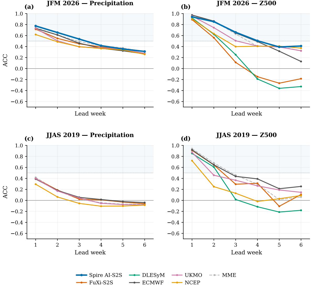
Figure 2: All-India anomaly correlation (ACC) versus lead week for six S2S systems. Top row: JFM 2026 (winter); bottom row: JJAS 2019 (monsoon). Columns: precipitation, Z500. Dotted line ACC= 0.5; solid line ACC= 0; shaded band marks ACC \geq 0.5. DLESyM provides no precipitation; Spire is unavailable for JJAS. The T2M comparison (three systems only) is shown in Figure 6.
