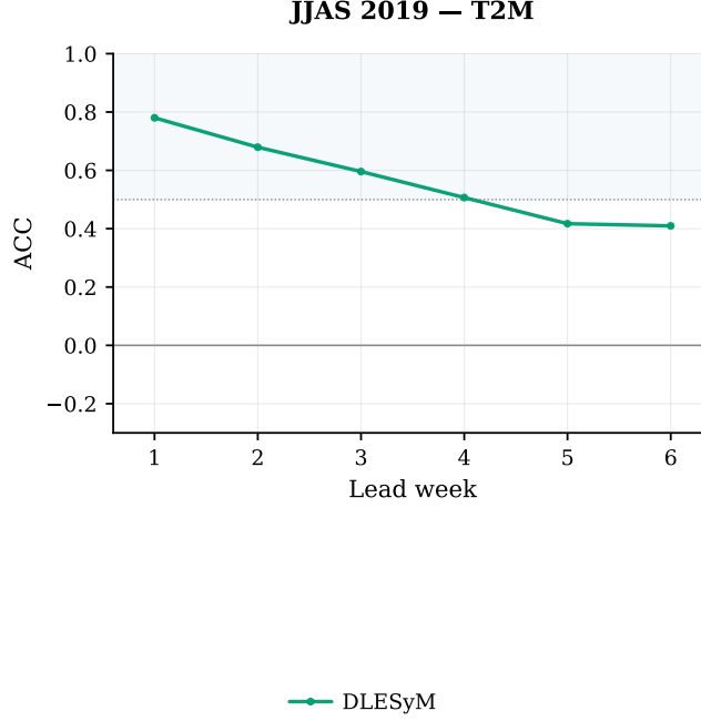
Figure 6: JJAS 2019 all-India T2M ACC versus lead week (DLESyM only; the only system with a scoreable T2M product in this season). The MME is identical to DLESyM here since no other system contributes.
