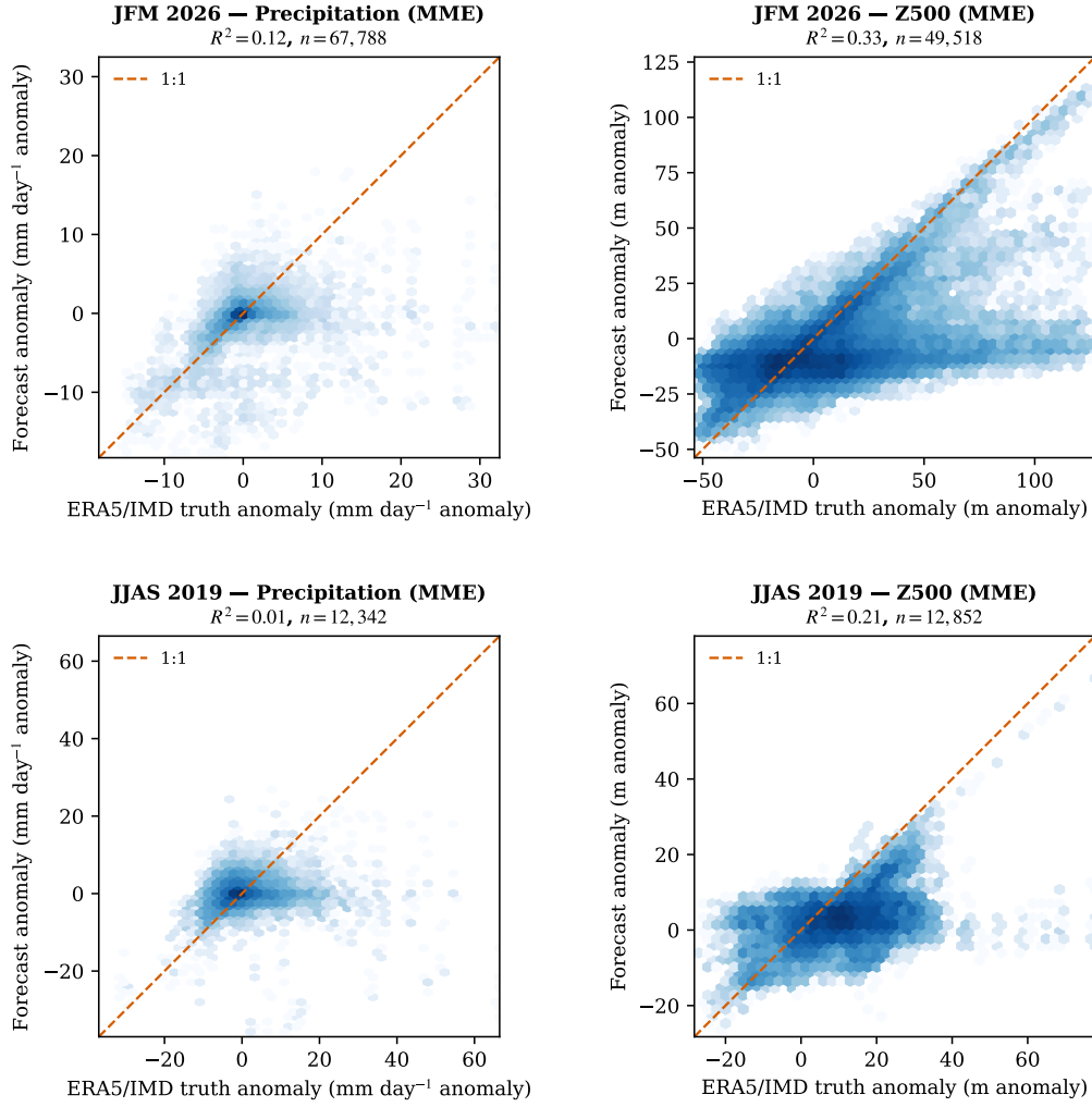
Figure 9: Forecast versus observed weekly anomaly for the multi-model ensemble (MME), pooled over all grid cells, lead weeks 1–6, and initializations. Hexbin shading shows point density (log scale); the dashed line is the 1:1 reference. R^2 is the squared Pearson correlation of the pooled pairs.
