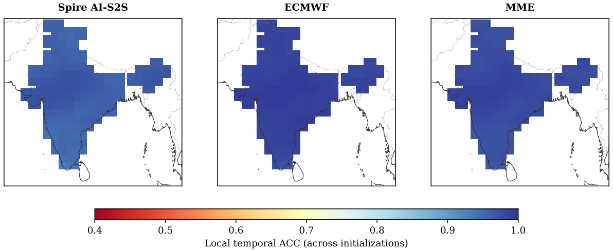
Figure 8: As Figure 7 but for week-1 Z500 anomaly. Note the different color scale (0.4–1.0 versus –0.4–1.0 for precipitation), reflecting the much higher and more spatially uniform circulation skill.
