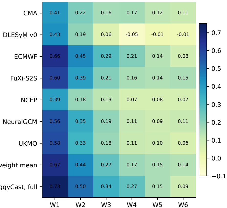
Spatial ACC (higher is better)
