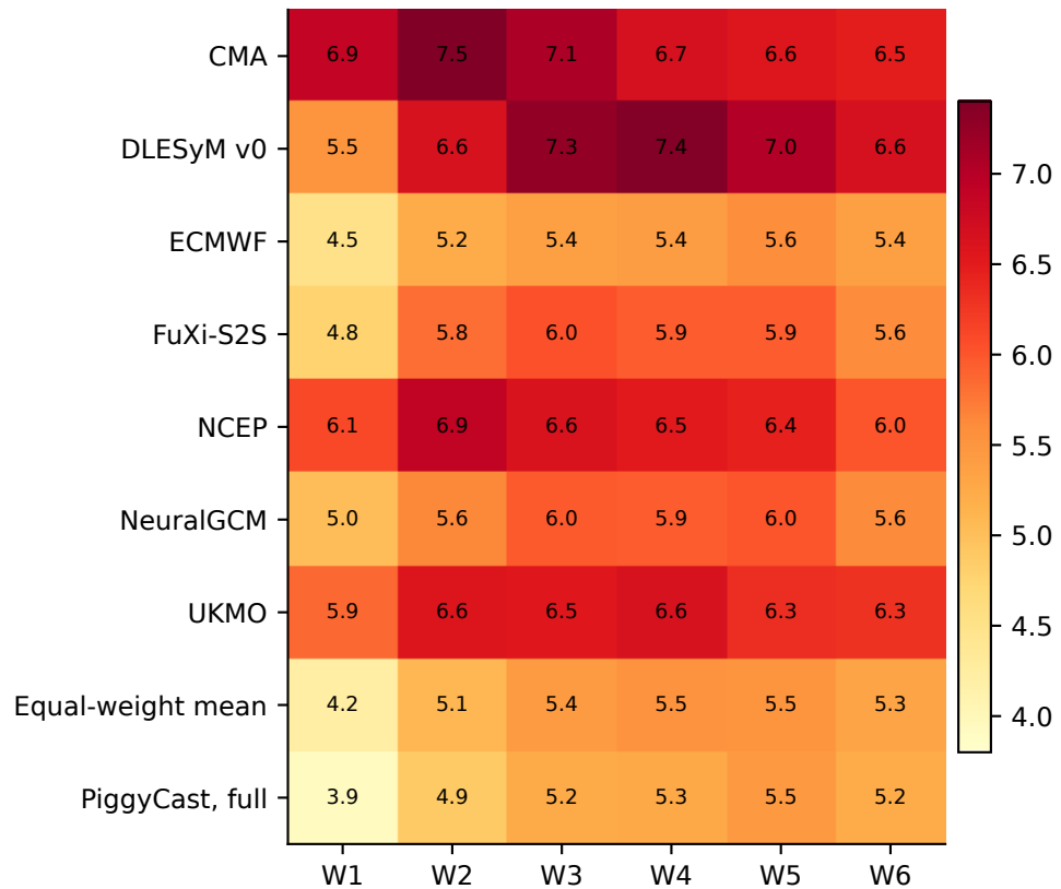
RMSE, mm day -1 (lower is better)
