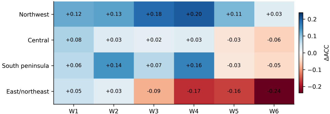
Full PiggyCast minus equal-weight spatial ACC
