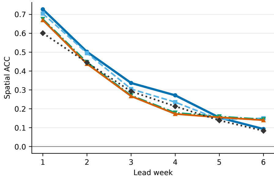
(a) Anomaly-pattern skill
