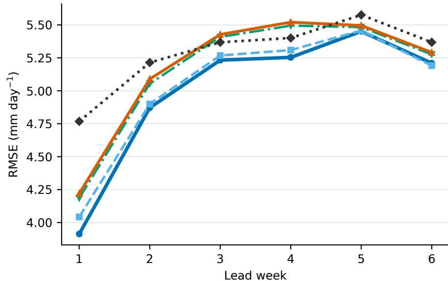
(b) Rainfall amount error
