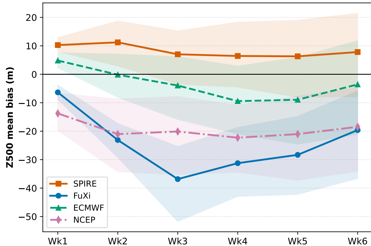
(a) Z500 mean bias vs lead
