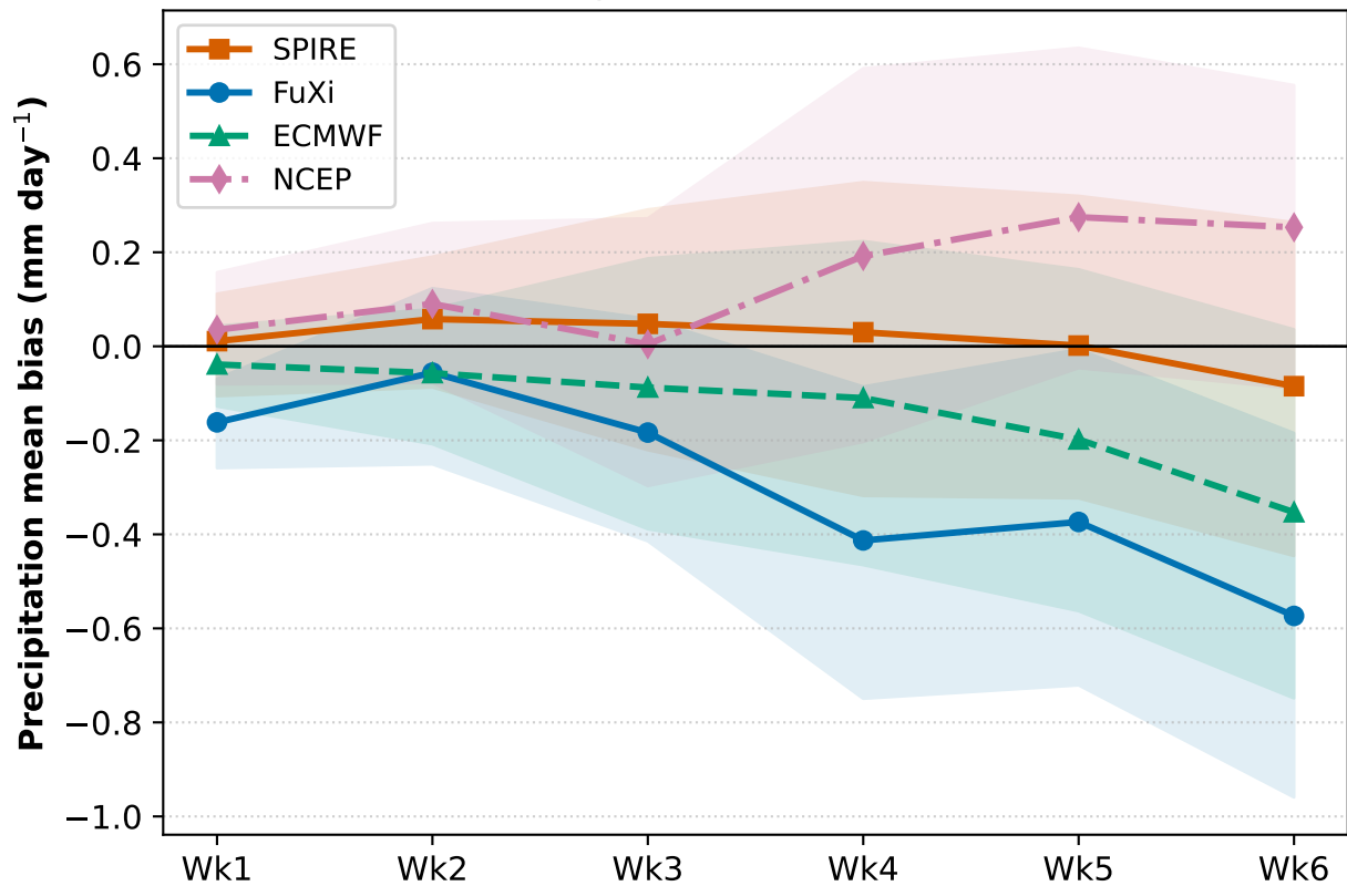
(b) Precipitation mean bias vs lead
