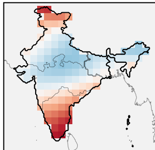
NCEP
