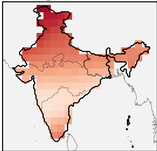
Spire AI-S2S
