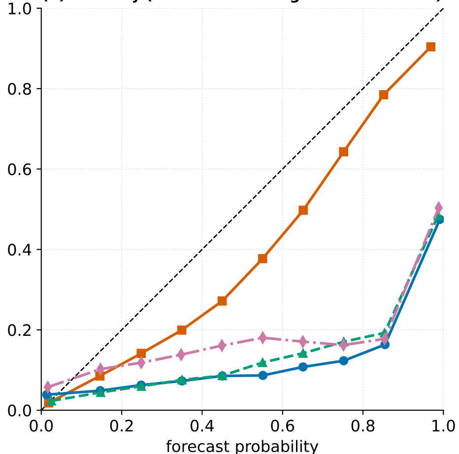
(b) Cold day (T2M < climatological lower tercile)
