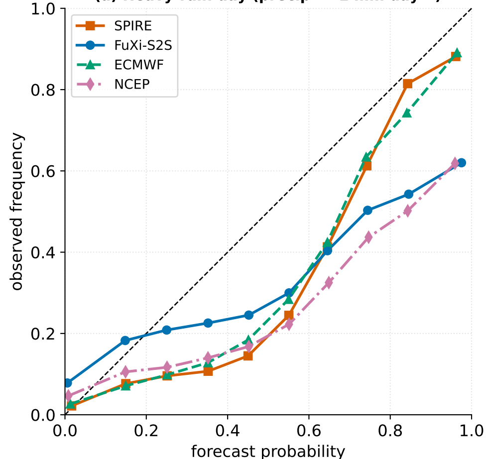
(a) Heavy-rain day (precip > 1 mm day -1 )
