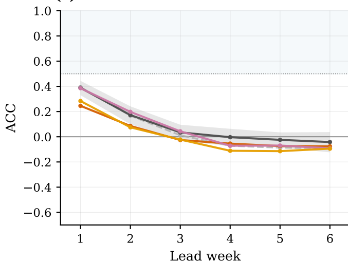
JJAS 2019 — Precipitation
