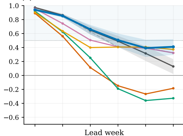
JFM 2026 — Z500
