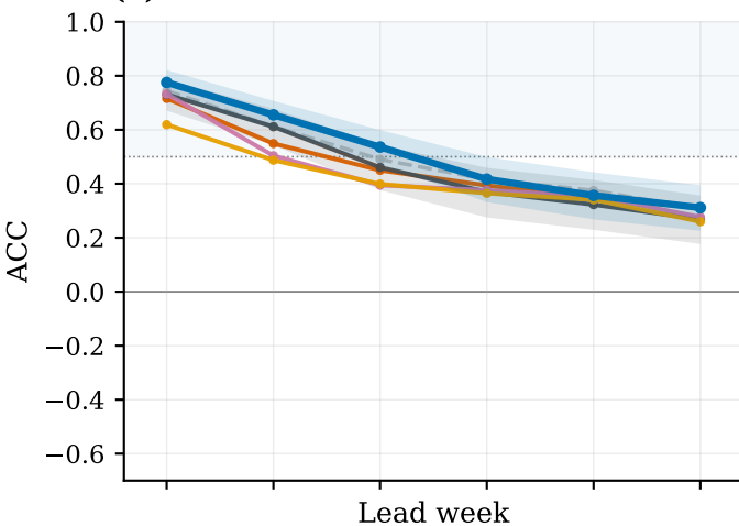
JFM 2026 — Precipitation
