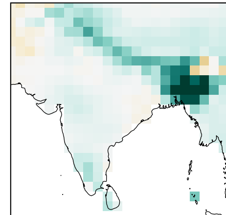
NCEP
