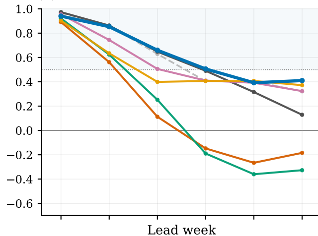
JFM 2026 – Z500
