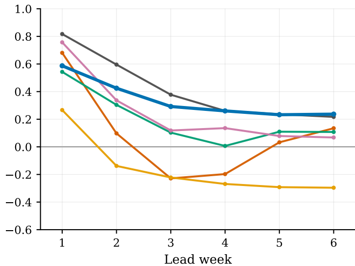
(b) JFM 2026 CRPSS — Z500
