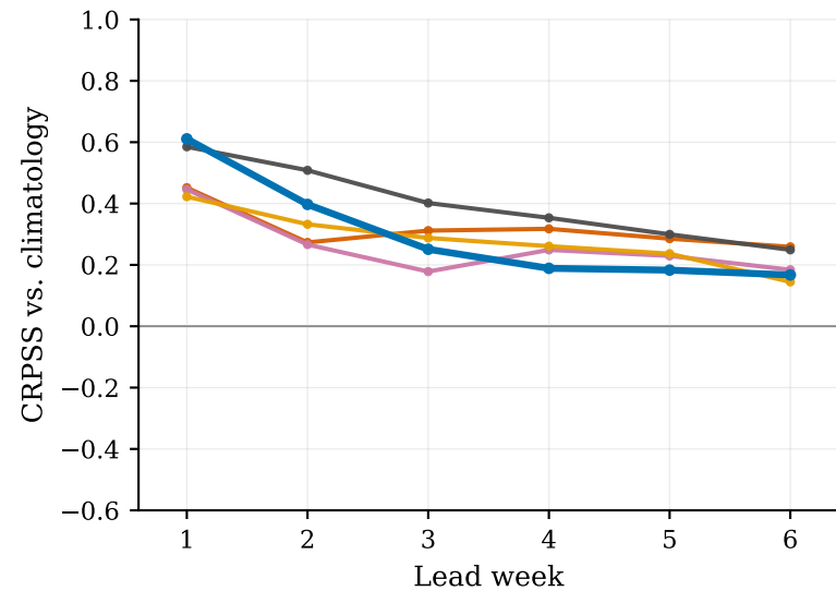
(a) JFM 2026 CRPSS — Precipitation
