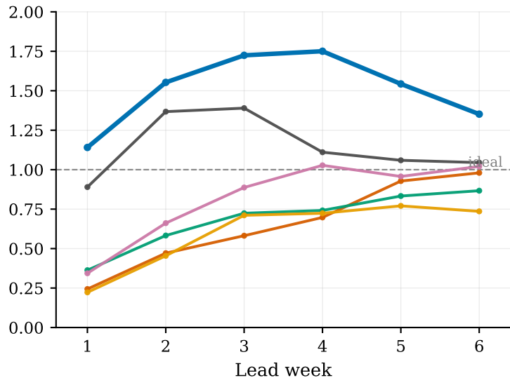
(b) JFM 2026 spread-skill — Z500
