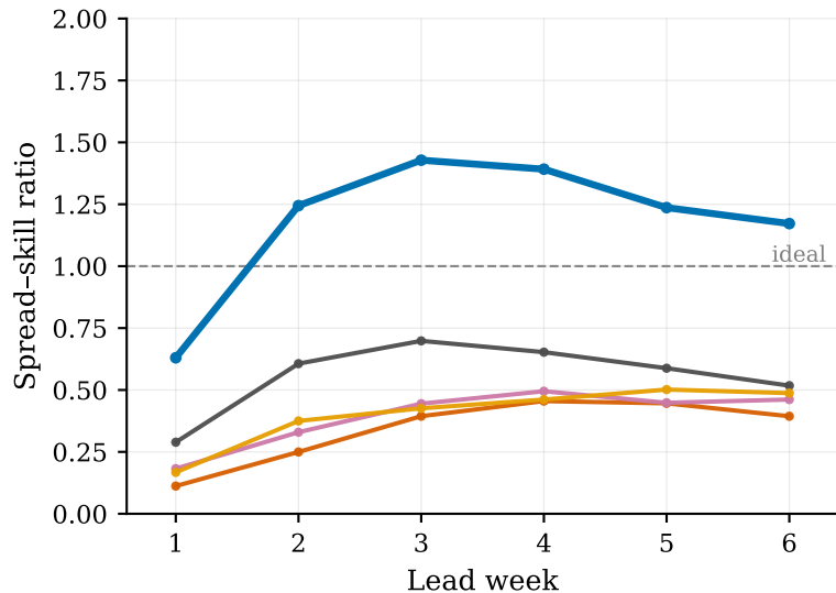
(a) JFM 2026 spread-skill — Precipitation
