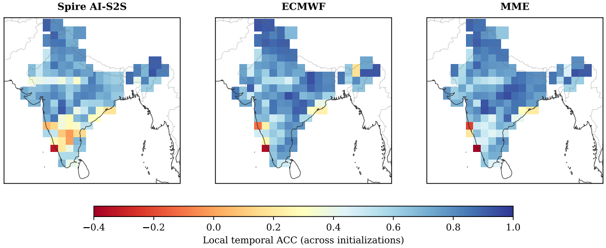
Figure 7: Local temporal ACC (Pearson correlation across the 90 JFM 2026 initializations) for week-1 precipitation anomaly at each 1.5° grid cell, for Spire AI-S2S, ECMWF, and the multi-model ensemble (MME). All three systems are weakest over the southern tip of the peninsula.
