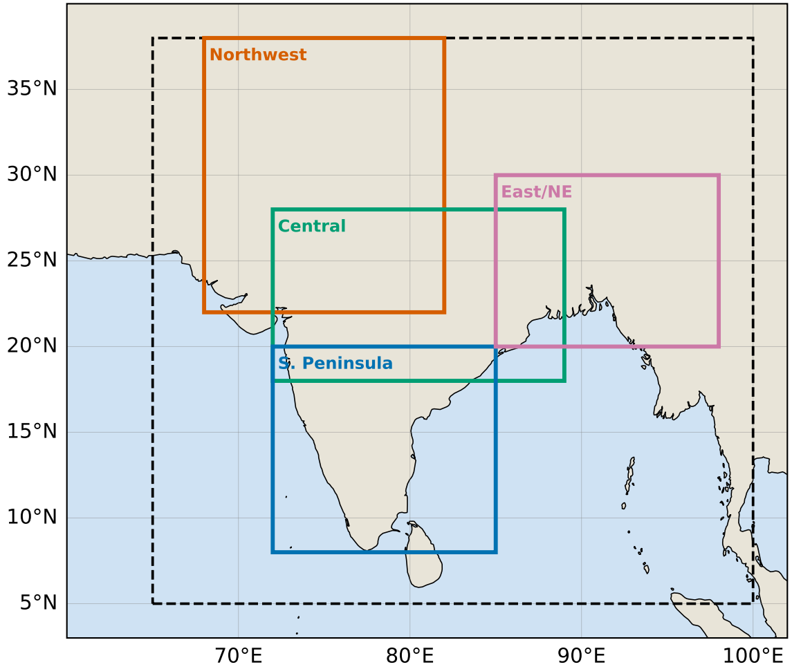
India verification domain (5–38°N, 65–100°E) and IMD homogeneous regions 13 weekly initializations, 1 Jan – 26 Mar 2026 · land points only
