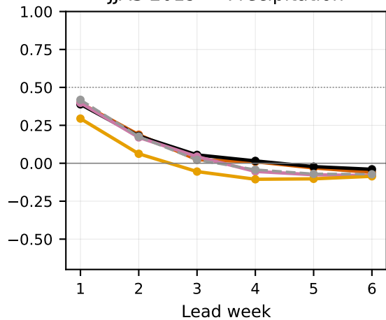
JJAS 2019 — Precipitation
