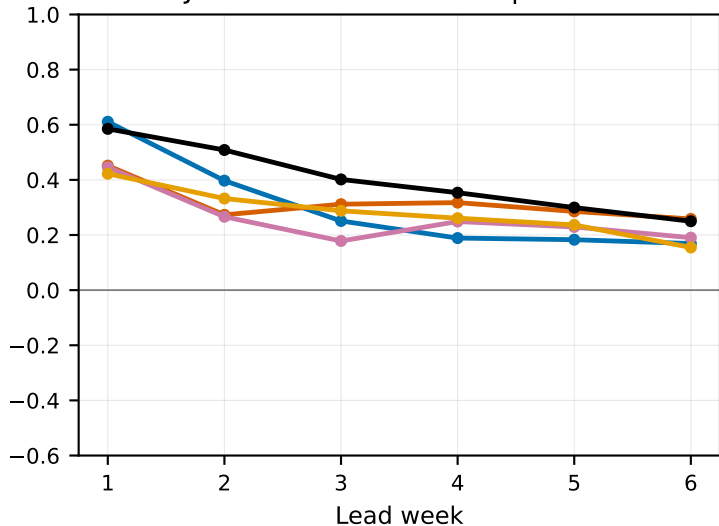
JFM 2026 CRPSS — Precipitation
