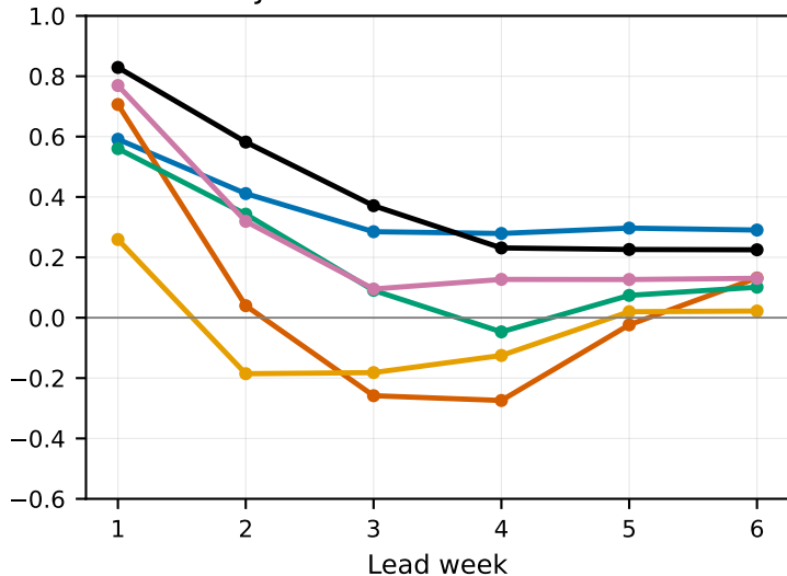
JFM 2026 CRPSS — Z500
