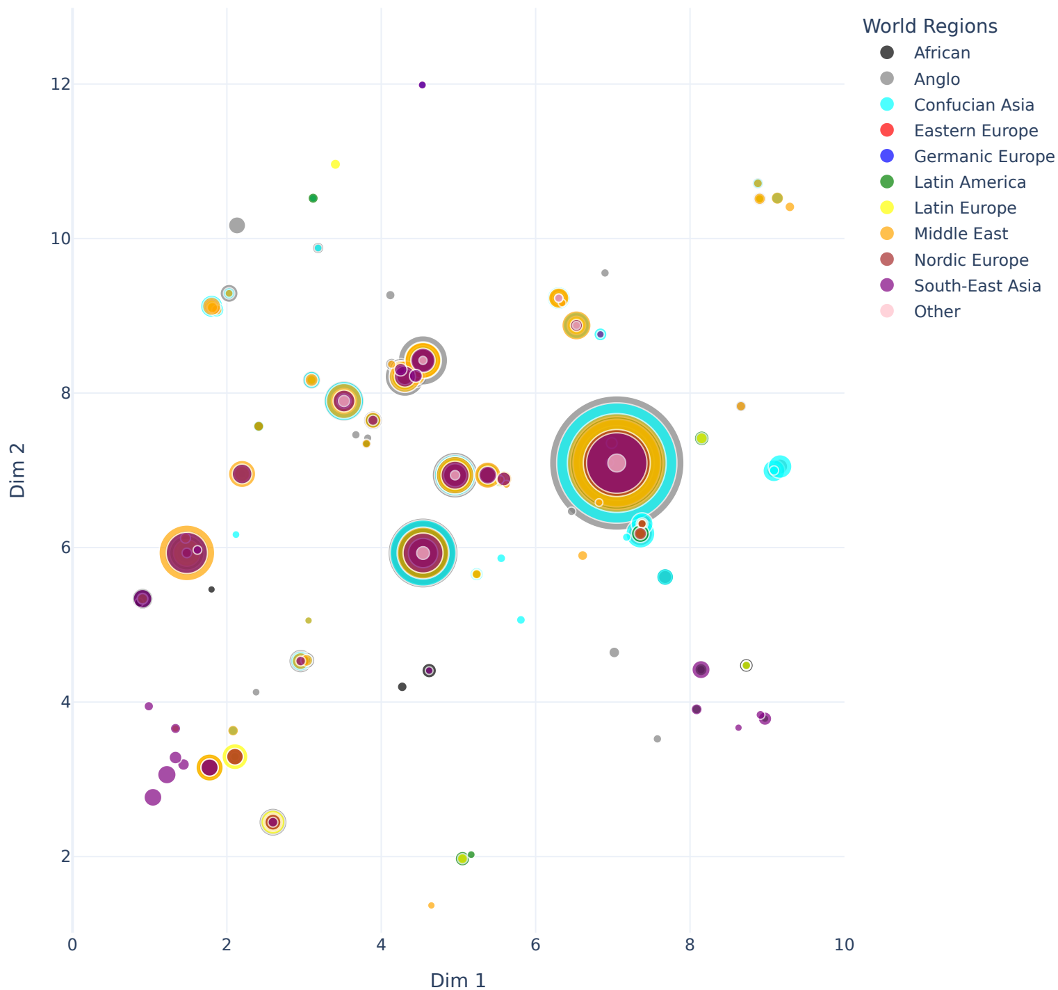
Qwen2.5-VL-7B-Instruct Region-wise Activity Semantic Map
