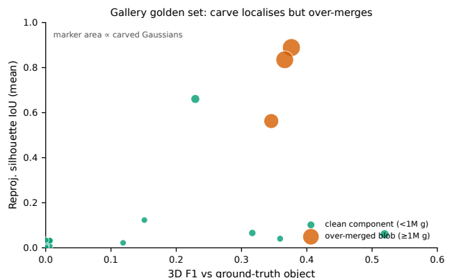
Figure 3: Carve localises but over-merges where a class tiles the scene. Marker area \propto carved Gaussians.
