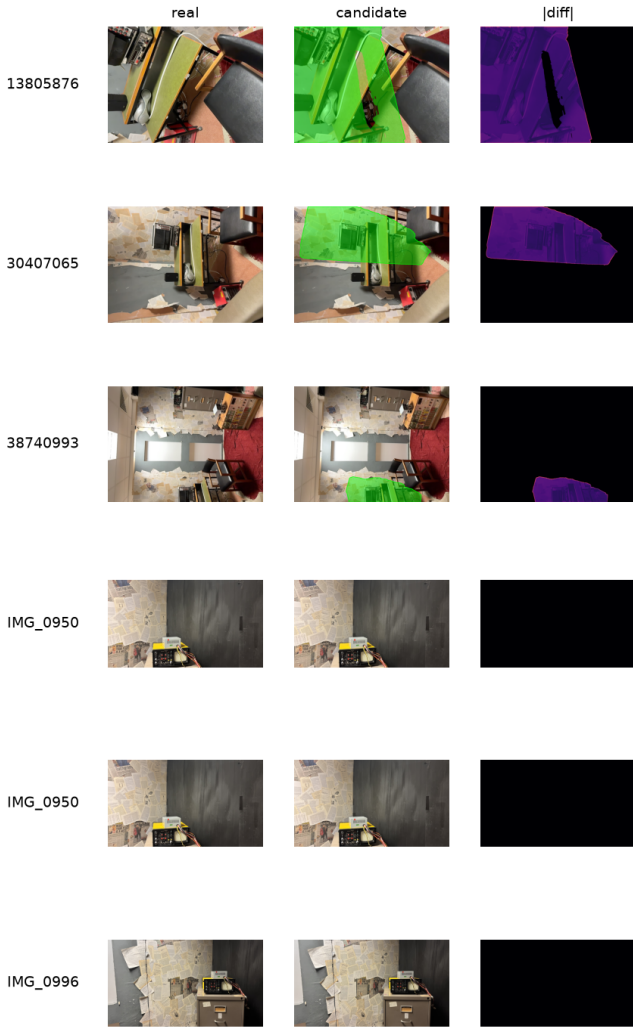
Figure 12: Per-camera evidence for the Lane-A radio: real frame, candidate silhouette (green) and absolute difference, across six real cameras. Where the green spills onto walls and furniture the carve has over-captured, which is why absolute silhouette IoU is not yet a reliable lane score.
