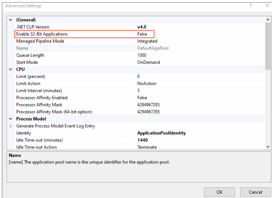
Figure: Advanced Settings of the DefaultAppPool
