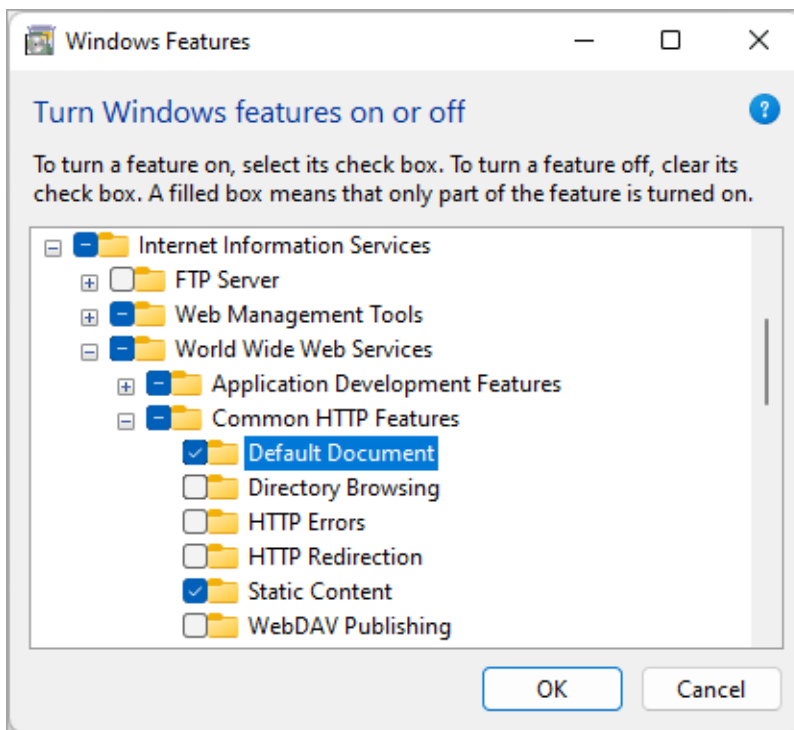
Figure: Enabling of the Common HTTP Features
