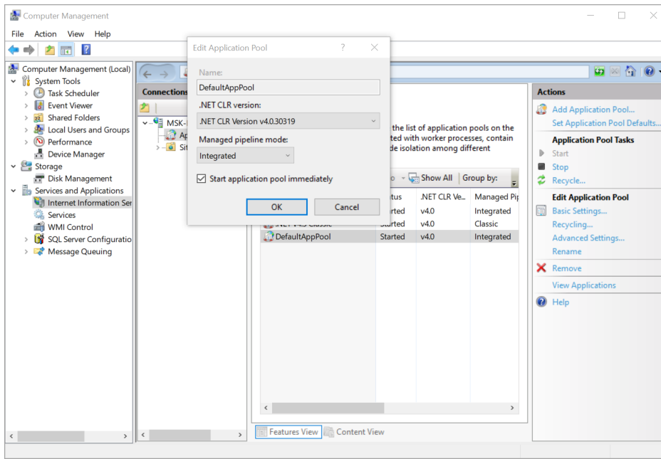
Figure: The settings of the default application pool
