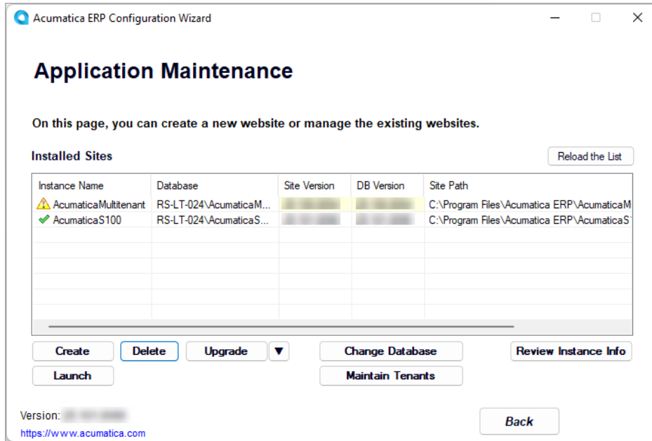
Figure: The updated list of instances
