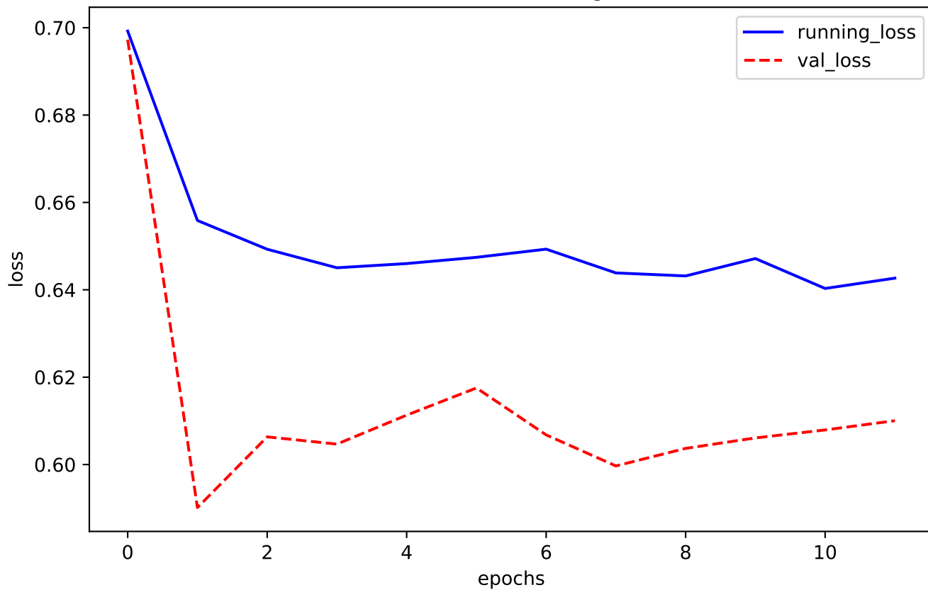
validation vs running loss
