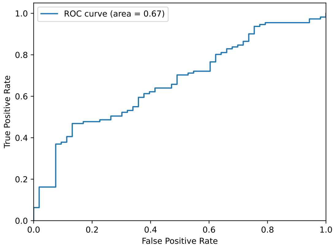
ROC Curve for linear model
