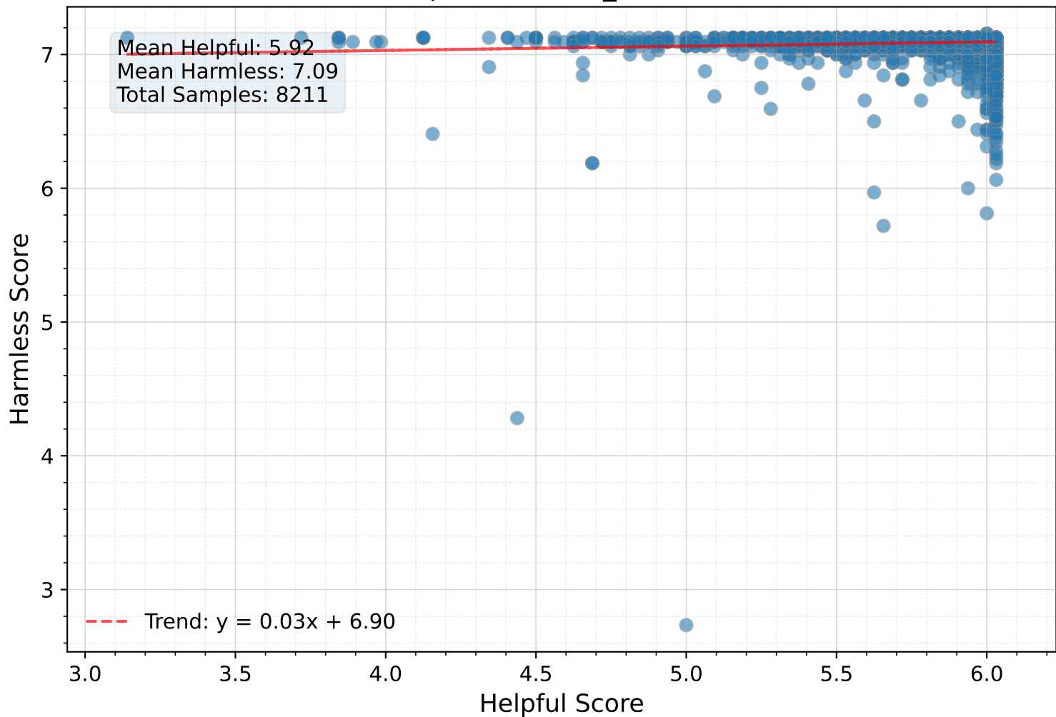
Score Distribution: Helpful vs Harmless (qwen2.5-1.5b_vanilla)
