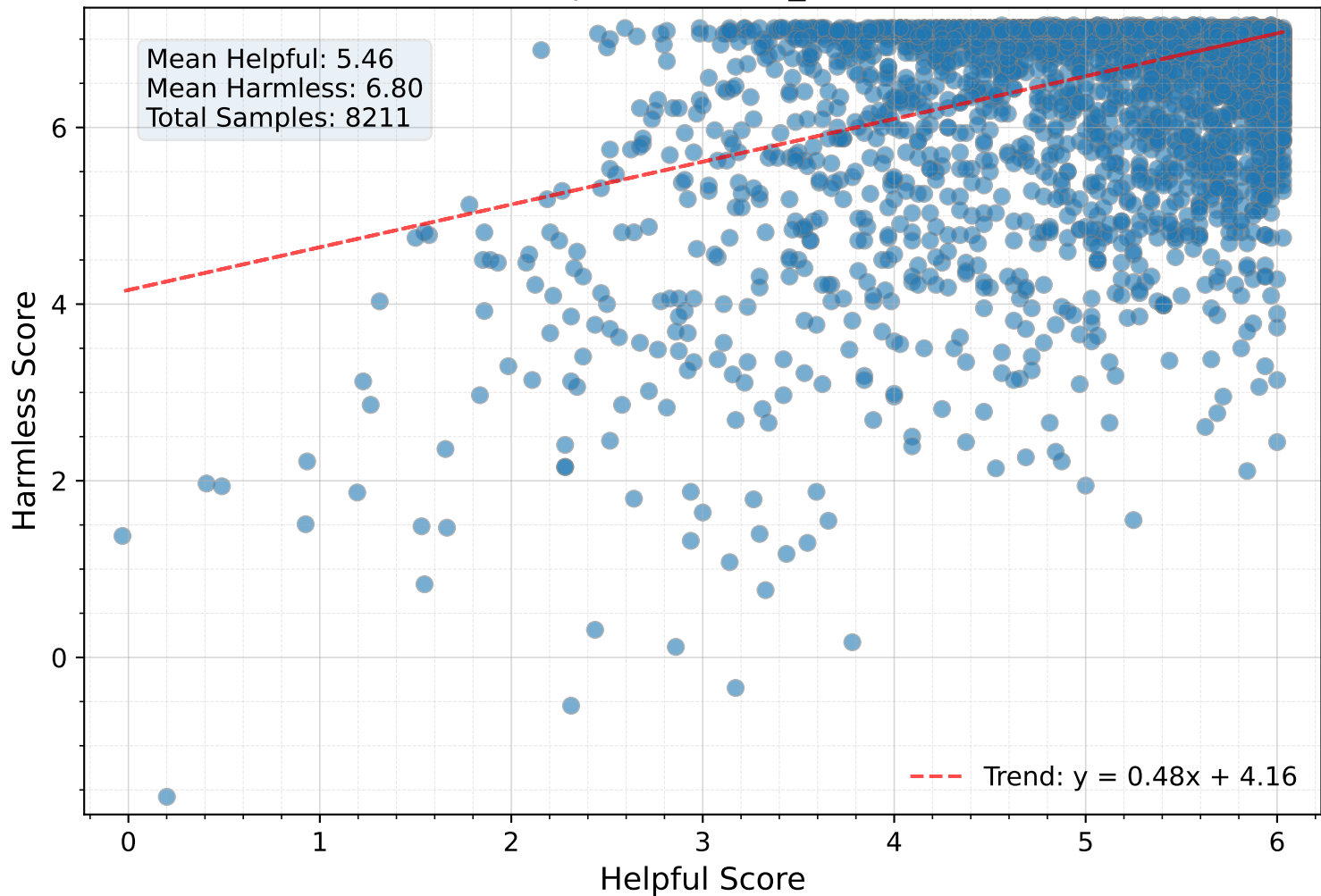
Score Distribution: Helpful vs Harmless (qwen2.5-1.5b_hv)
