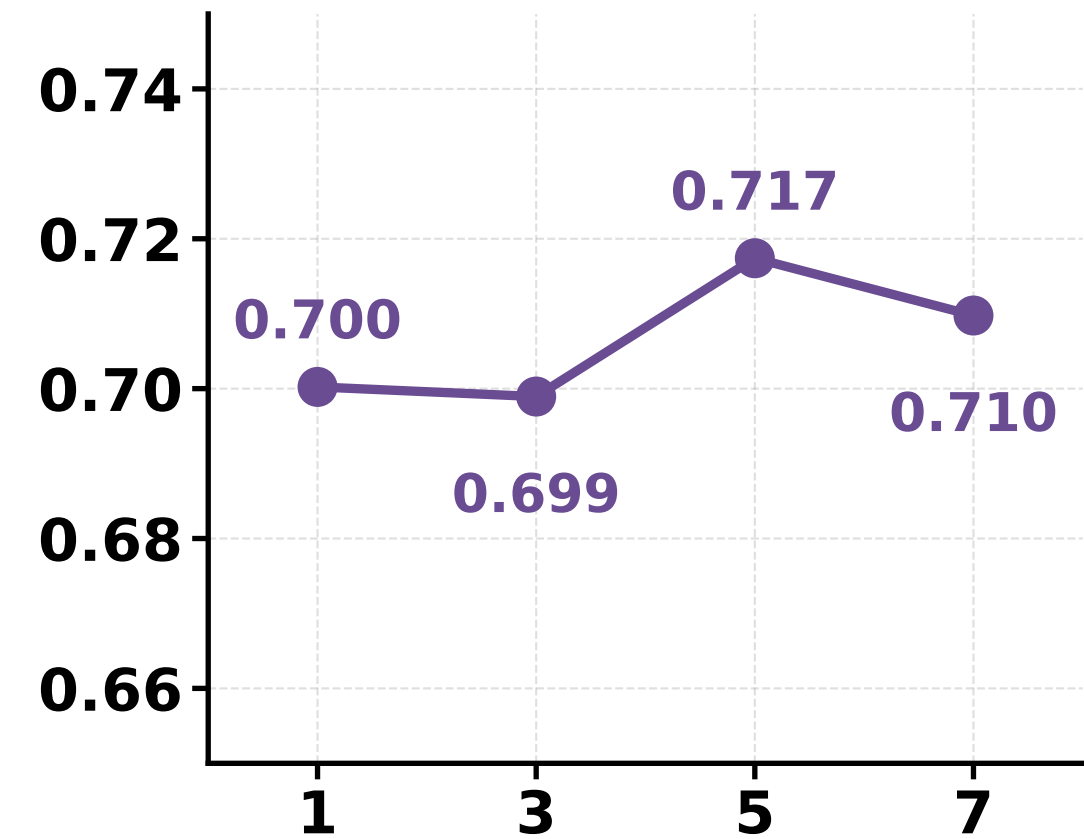
Hypervolume
