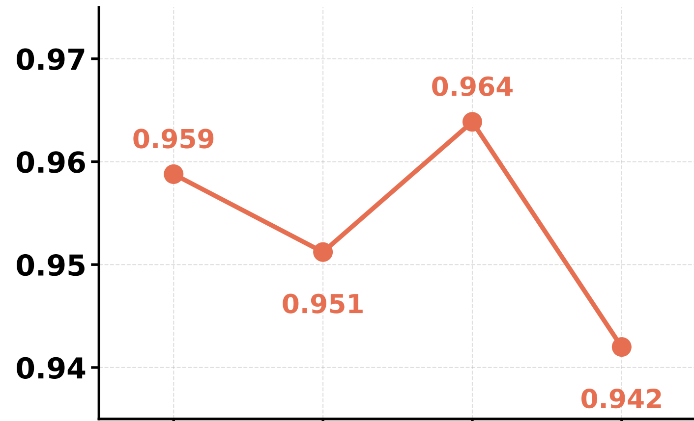
Conciseness
