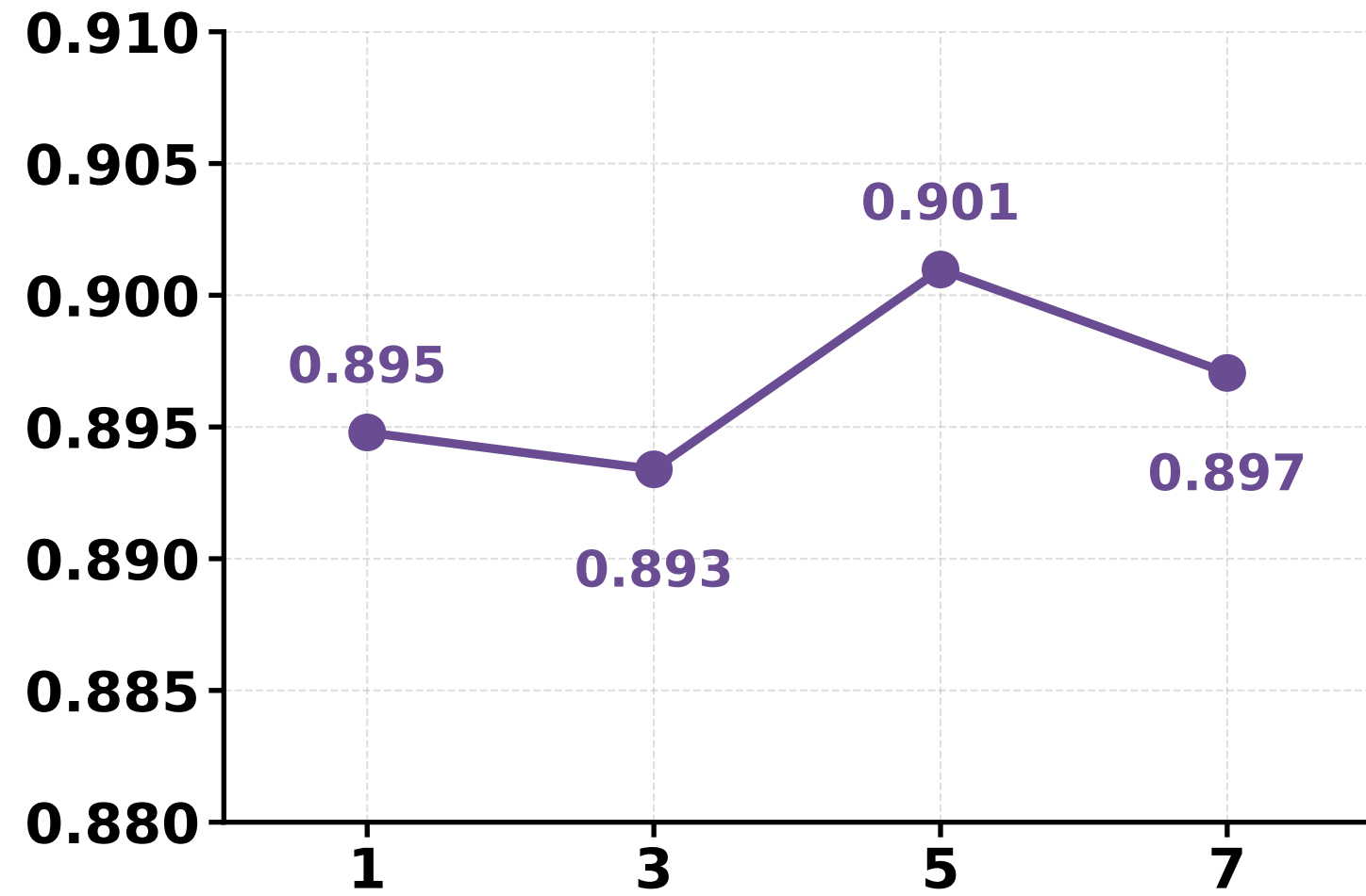
Overall
