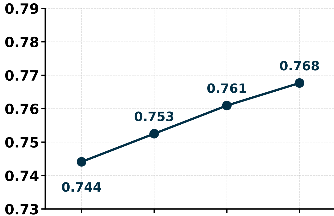
Correctness
