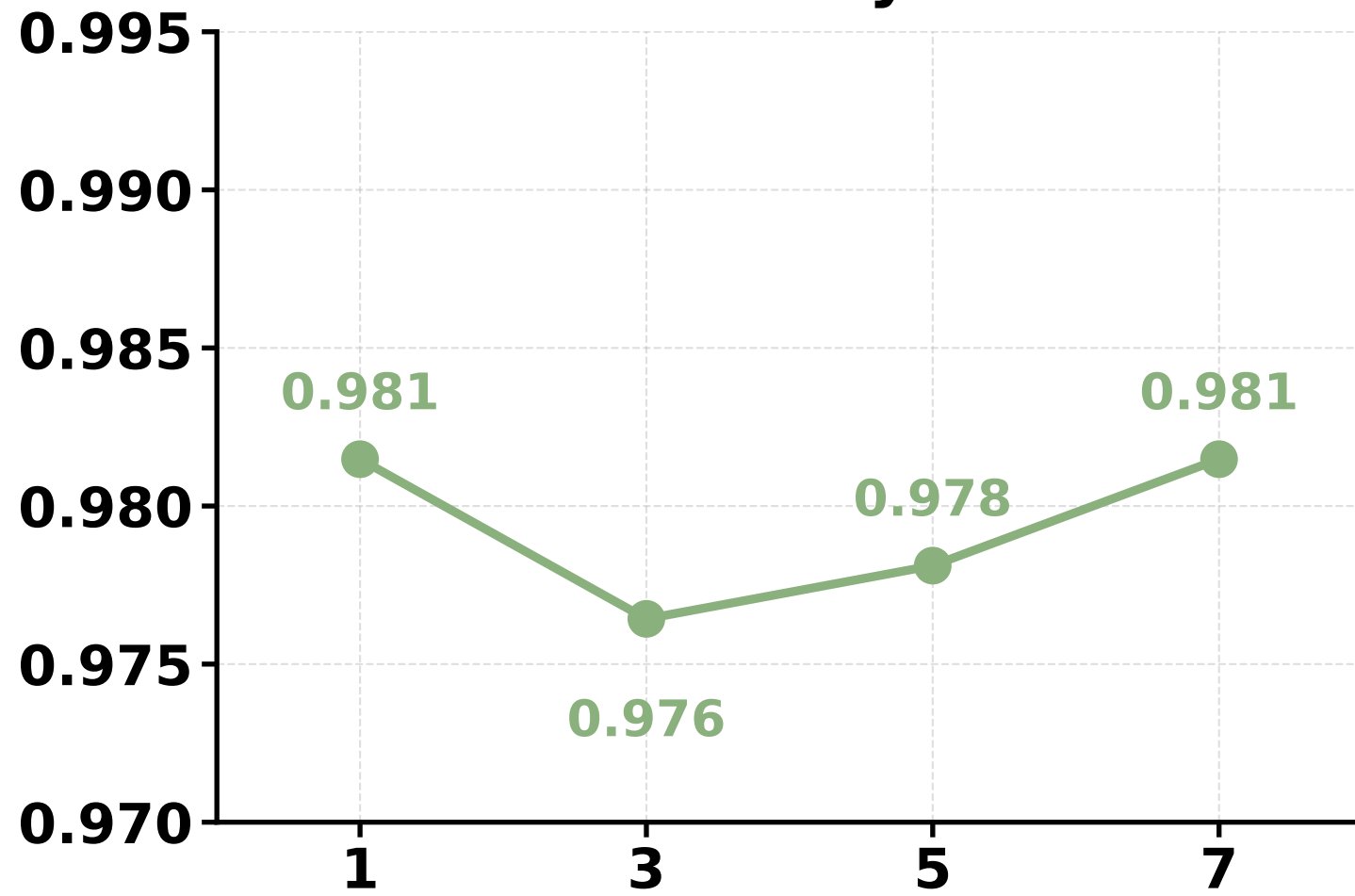
Clarity
