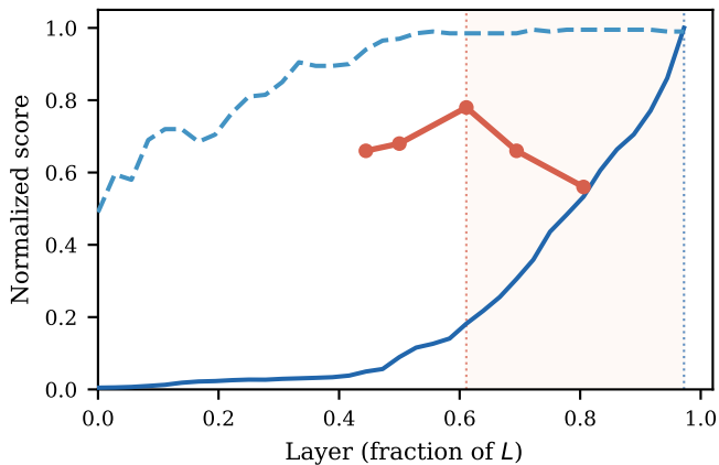
Qwen3-8B (gap: 36%)
