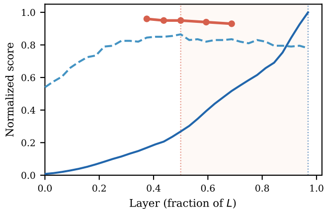
Gemma-3-27B (gap: 26%)
