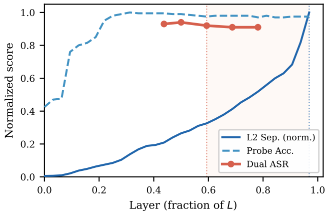
Qwen3-8B (gap: 36%)
