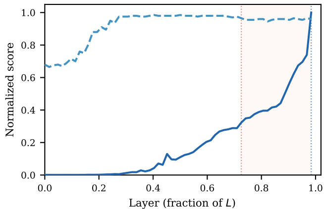
Gemma-3-27B (gap: 26%)
