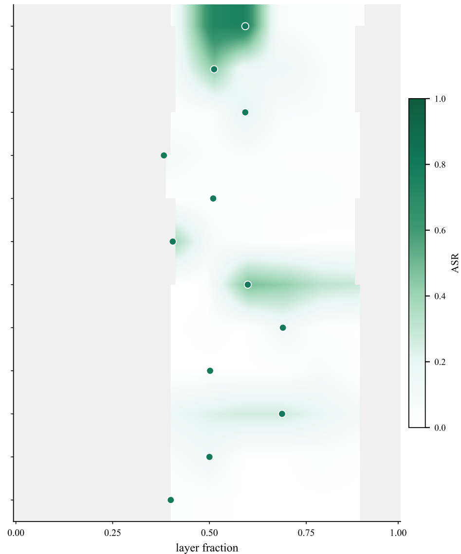
Ablation-only ASR over baseline (controllability) peaks in the middle of the network
