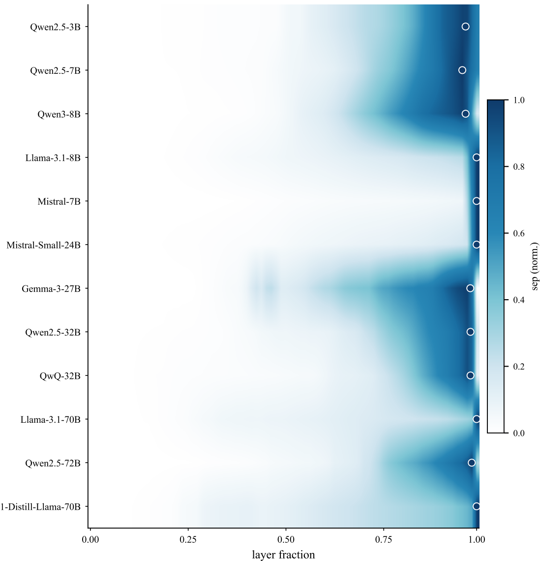
Separation (readability) — peaks at the final layer
